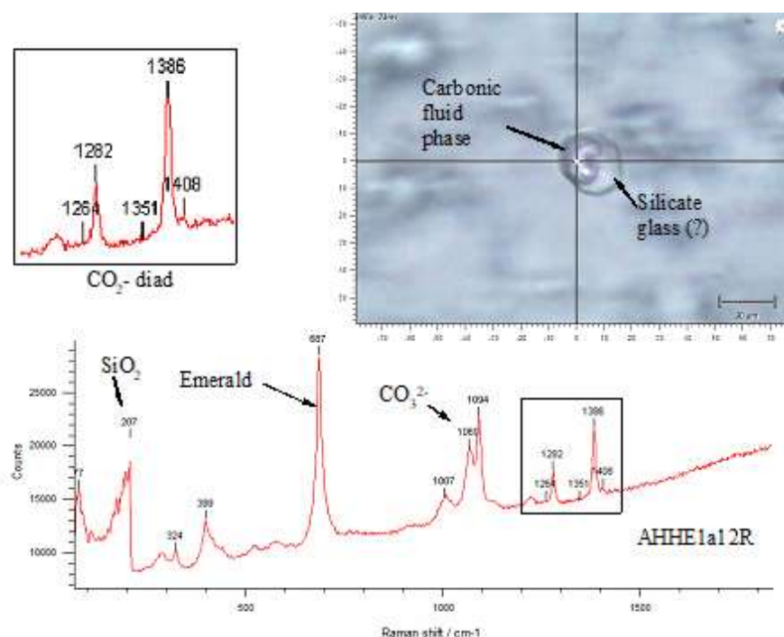
Fig. 5. Raman spectra of the fluid carbonic (liquid \text{CO}_2 + gas \text{CO}_2 ), and glassy silicate solid phase in emerald from Capoeirana. Informally, the calculated pressure of this inclusion based upon \text{CO}_2 diad (in medallion) with \Delta = +104 \text{ cm}^{-1} gives a calculated density of 0.479898 g/cm 3 (Lamadrid et al., 2017).
