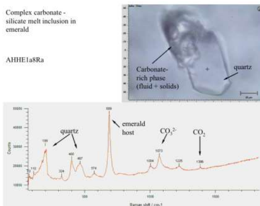
Fig. 4. Multiphase inclusion suggesting fluid-fluid-melt immiscibility at trapping conditions in emerald from Capoeirana.
