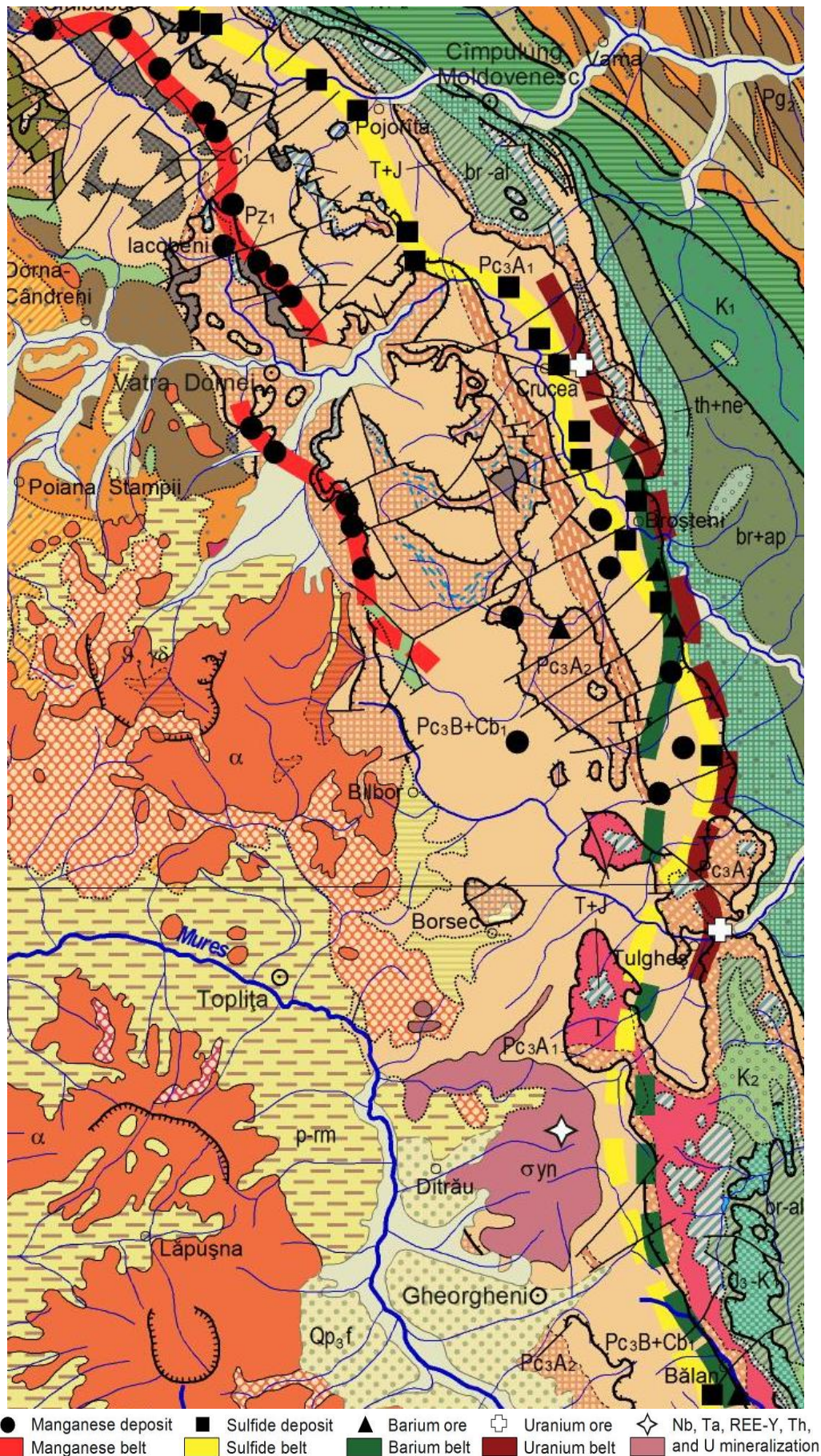
Fig. 1. Bistrița Mts with their 4 mineralized belts, localized in the Tulgheș Series: Mn, Ba, Sulfide, U, and Ditrău rare element minerals occurrence localized in Ditrău alkaline carbonatite complex.
