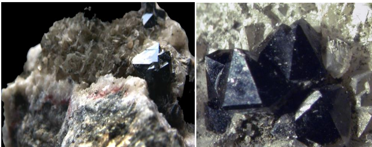
Fig. 21. Photo of uraninite crystals of 8mm size grown on/with calcite crystals in quartz gangue (grey) (left); Photo of uraninite crystal of 7mm grown on/with calcite crystals and with sulfide impregnation (right).
