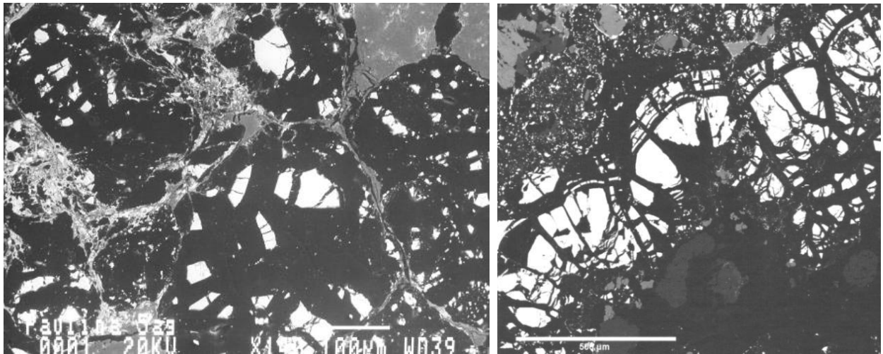
Fig. 18. Backscattered electron image of uraninite grains (bright white) in carbonaceous matter (black) and small sulfides (grey) intergrowth with coffinite (white) on veinlets (left); Backscattered electron image of botryoidal uraninite (bright white), coffinite (white, veinlets inside uraninite and around sulfides), carbonaceous matter (black), and sulfides (small grey grains, top left corner) (right).
