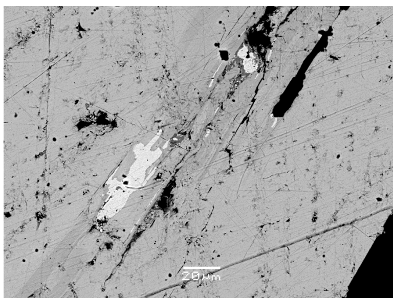
Fig. 3. Large-magnification SEM-BSE image showing the chemical composition heterogeneity of nagyagite as indicated by the existence of different gray tints. The whitish inclusions correspond to altaite and the black ones to native tellurium.
