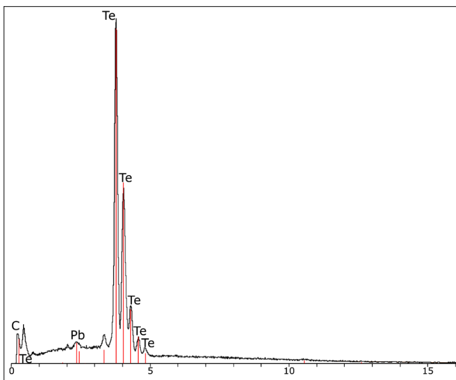
Fig. 5. SEM-EDS spectrum of native tellurium inclusion hosted by nagyagite from Săcărâmb.
