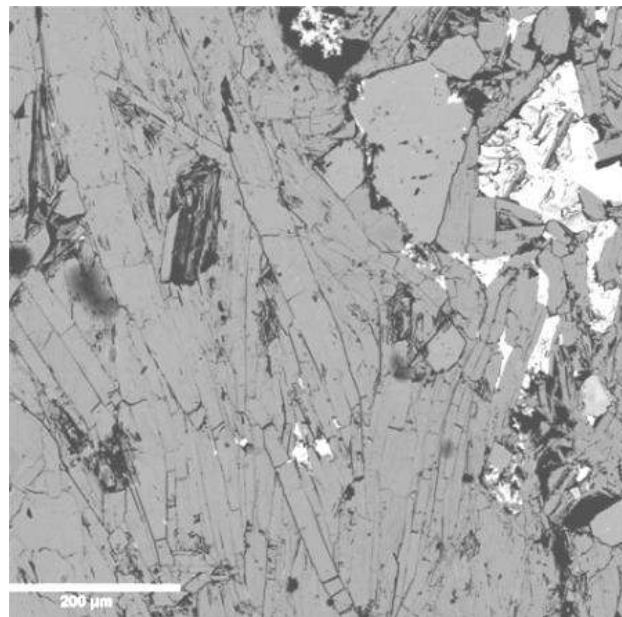
Fig. 15. Cymrite (large prisms, two cleavages), pyrite (black), and zircon (small, top), TL, NII, x30 (left); Backscattered electron image of cymrite (prisms, grey) and pyrite (white), Bălan deposit, Sulfide Belt.
