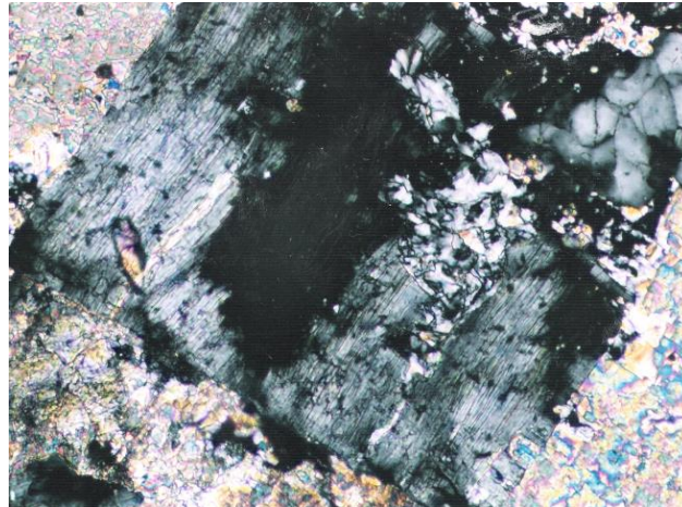
Fig. 16. Cymrite (large grey grains, perfect cleavage), partially altered, TL, N+, x30 (left); Cymrite (large quadratic shape) substituted by an amorphous mineral (black, isotrop), TL, N+, x35, Holdița deposit, Barium Belt.
