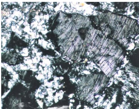
Fig. 16. Cymrite (large grey grains, perfect cleavage), partially altered, TL, N+, x30 (left); Cymrite (large quadratic shape) substituted by an amorphous mineral (black, isotrop), TL, N+, x35, Holdița deposit, Barium Belt.
