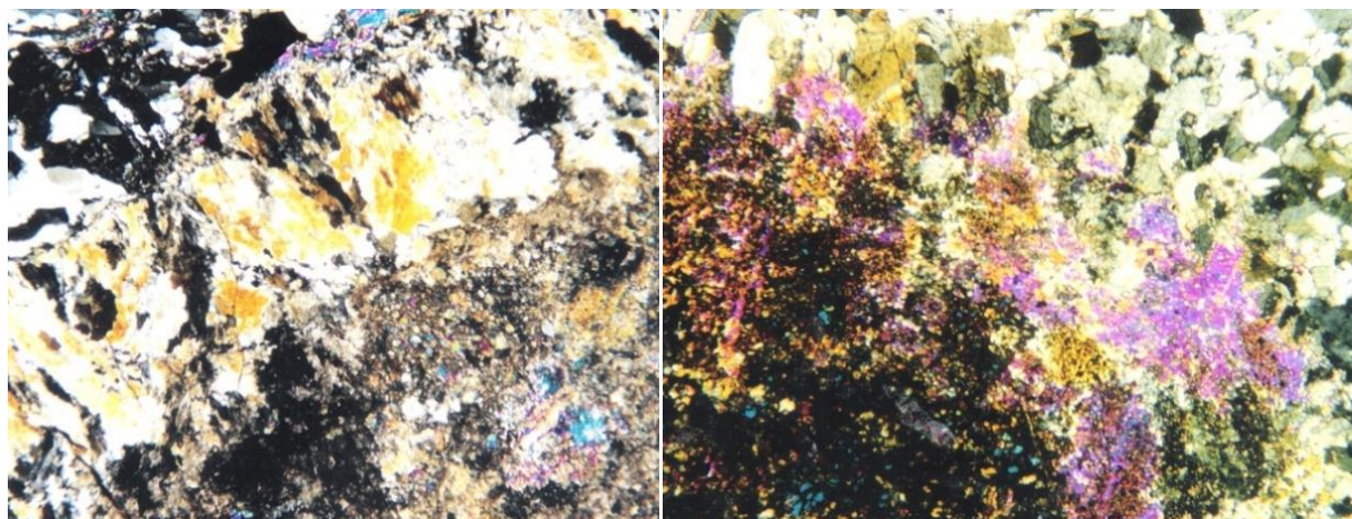
Fig. 3. Undersaturated paragenesis with no direct contact tephroite ore (bottom right corner)/quartzite country rock (top left corner), between them always there is a rhodonite band (centre, white yellow), TL, N+, x20 (left); Undersaturated paragenesis: tephroite substituted by manganpyrosmalite (bottom, left corner), rhodonite (top, right corner) and manganpyrosmalite vein between them (centre), TL, N+, x25 (right).
