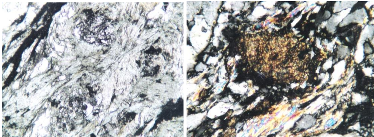
Fig. 17. Pietrosu Bistriței porphyroide granite: almandine relics in quartz/chlorite/albite/graphite rock, TL, NII, x30. Titanite (centre), muscovite (cleavage, colored), quartz (white-grey), and albite (white), TG4 level (left);
