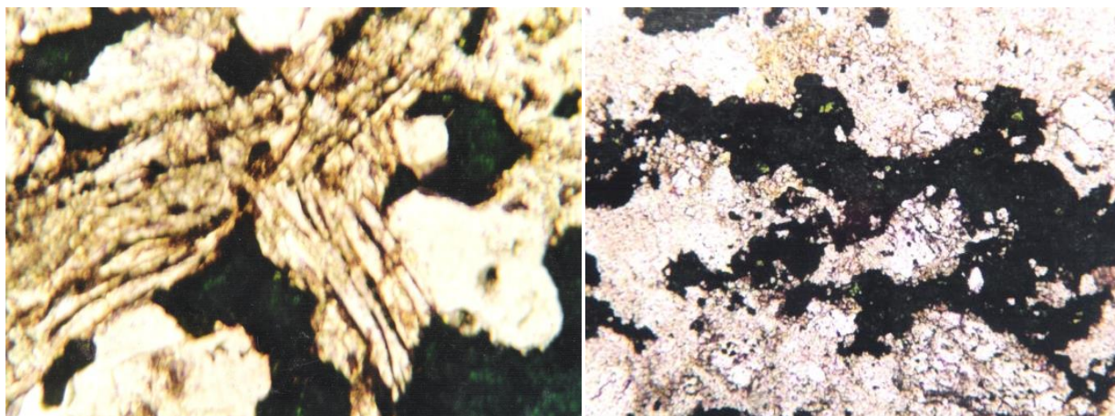
Fig. 9. Alabandite (green), kinoshitalite (large grain, light yellow) and celsian (white), TL, NII, x30, Barium Belt. Alabandite (dark green), Mn-humite (white pinkish), and rhodochrosite (white), TL, NII, x35, Mangan Belt.
