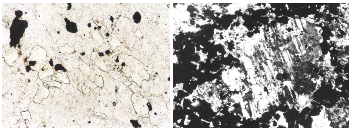
Fig. 7. Celsian (white, relics) and pyrite (black) in barite ore (pinkish white), TL, N+, x30, Barium Belt (left); Celsian (twinned, centre) and pyrite (black, around), TL, N+, x35, Sulfide belt (right).
