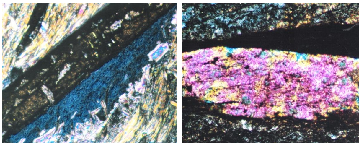
Fig. 14. Rutile (large yellow brown prism crystal), clinocllore (blue, anomaly birefringence), and muscovite (colored, cleavage), TL, N+, x25, sample Prs3, Pârâul Șarpe deposit, Sulfide Belt (left); Epidote (large crystal, high birefringence) with ilmenite around it (dark brown, black) enclosed in micaceous chloritized rock, TL, N+, x30, Pârâul Șarpelui deposit, Sulfide Belt (right).
