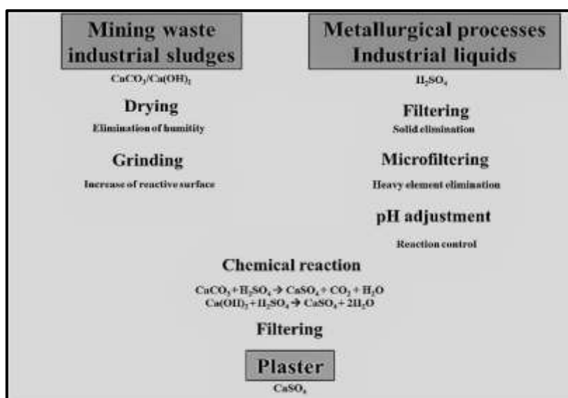
Fig. 2. Flowchart of plaster (Ecogypsum®) production.
