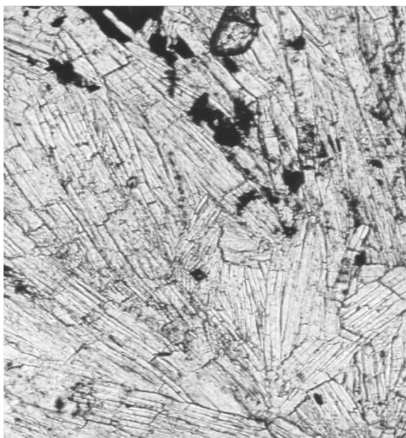
Fig. 15. Cymrite (large prisms, two cleavages), pyrite (black), and zircon (small, top), TL, NII, x30 (left); Backscattered electron image of cymrite (prisms, grey) and pyrite (white), Bălan deposit, Sulfide Belt.
