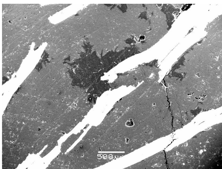
Fig. 2. Large-field SEM-BSE image of nagyagite lamellas hosted by rhodochrosite from Săcărâmb ore deposit.
