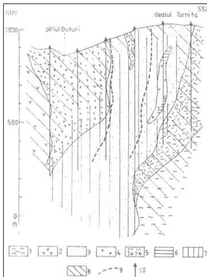
Fig. 2. Geological sketch section of Bucium Tarnita deposit (Popescu, 1986): 1. Cretaceous sedimentary rocks, 2. Arama type andesites, 3. Tarnita type andesite (periphery), 4. Tarnita type andesite (central), 5. Breccias: a. andesitic, b. sedimentary, 6. Alkali feldspar – chlorite (biotite) zone, 7. Sericite – argillic minerals zone, 8. Chlorite – calcite – epidote zone, 9. Cupriferous impregnation limit, 10. Drills.
