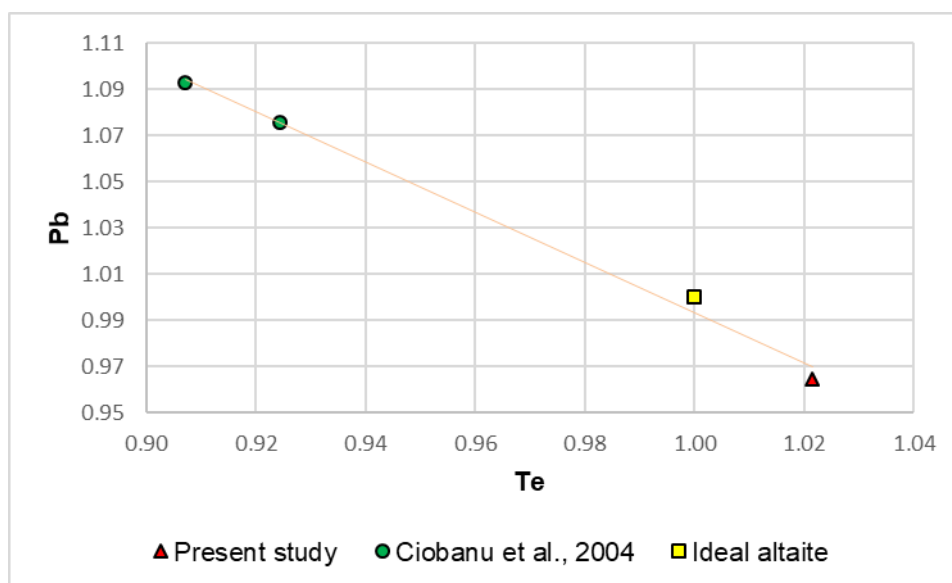
Fig. 6. Plot of different altaite compositions from the literature, the present study, and the ideal composition in terms of Pb vs. Te (apfu). The brown line marks a negative correlation trend.
