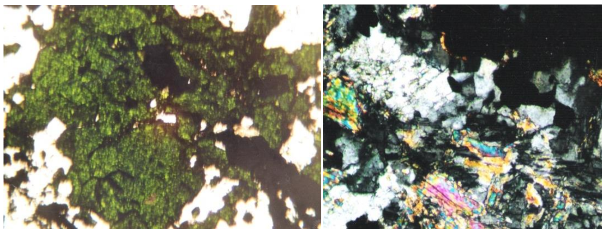
Fig. 10. Alabandite (green), celsian (white), and pyrite (black), TL, NII, x35, sample GB2, Sulfide Belt (left); Kinoshitalite (high birefringence, cleavage), celsian (white), and pyrite (black), TL, N+, x30, Ba-Belt.
