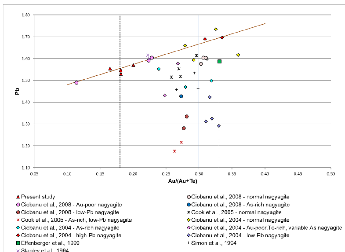
Fig. 7. Plot of different nagyagite compositions (recalculated based on 5 apfu) from the literature and the present study onto \Sigma\text{Pb} vs. \text{Au}/(\text{Au}+\text{Te}) diagram (Ciobanu et al., 2004). The dotted lines mark the average values of \text{Au}/(\text{Au}+\text{Te}) ratios for the “ normal nagyagite ” and for the nagyagite from the present work; the blue line highlights the constant value for \text{Au}/(\text{Au}+\text{Te}) ratio, and the brown line marks a positive correlation trend.
