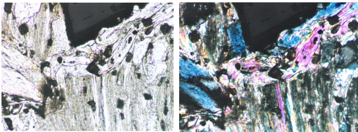
Fig. 13. Anandite (micaceous) with Ti mineral and uraniferous zircon inclusions, and zoned pyrite (top, black), TL, NII, x30 (left); The same image in N+ (right), sample Bln1, Bălan deposit, Sulfide Belt.
