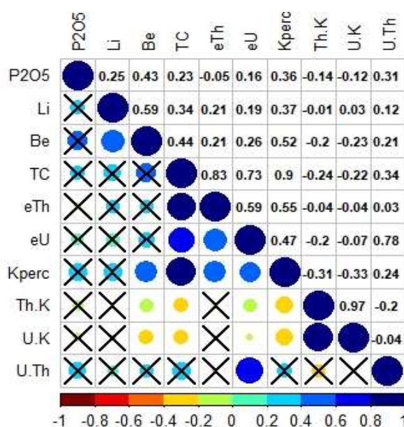
Fig. 2. Pearson’s correlation matrix between Li, Be, P with gamma-ray spectrometric data.
