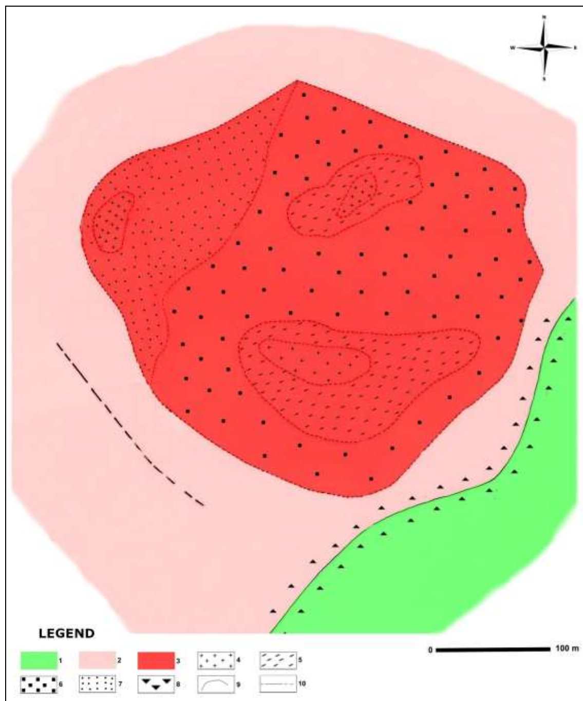
Fig. 3. Schetch map of +880 m level of Bucium Tarnita exploitation showing the main alteration patterns (modified after Bostinescu, 1983). 1. Albian deposits, 2. Tarnita andesites (lava), 3. Tarnita andesites (stock), 4. Tarnita andesites (central unaltered deep facies), 5. Phyllic alteration zone, 6. Potassic alteration zone, 7. Argillic zone, 8. Breccia, 9. Geological boundary, 10. Vein.
