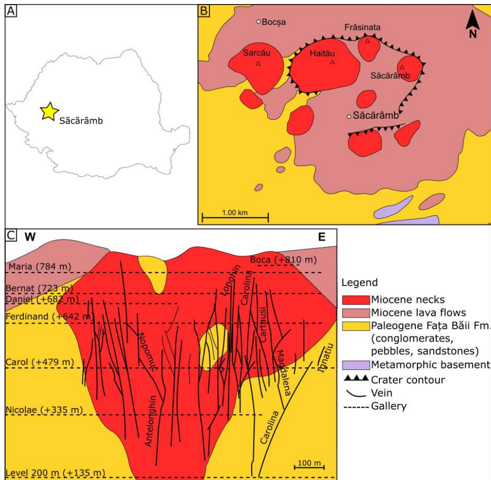
Fig. 1. Simplified geology of Săcărâmb area (a) and the location of the main veins and mining levels (Ciobanu et al., 2004 and 2008).
