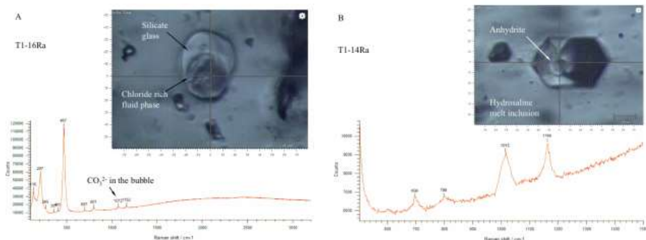
Fig. 5. Raman spectra of the same complex silicate-hydrosaline melt inclusion pictured in Fig.4 showing the presence of carbonate ion in the bubble of the salt melt phase surrounded by silicate glass (A) and anhydrite daughter phase (B) formed in hydrosaline melt inclusion (without liquid phase at room temperature) from the same quartz sample.
