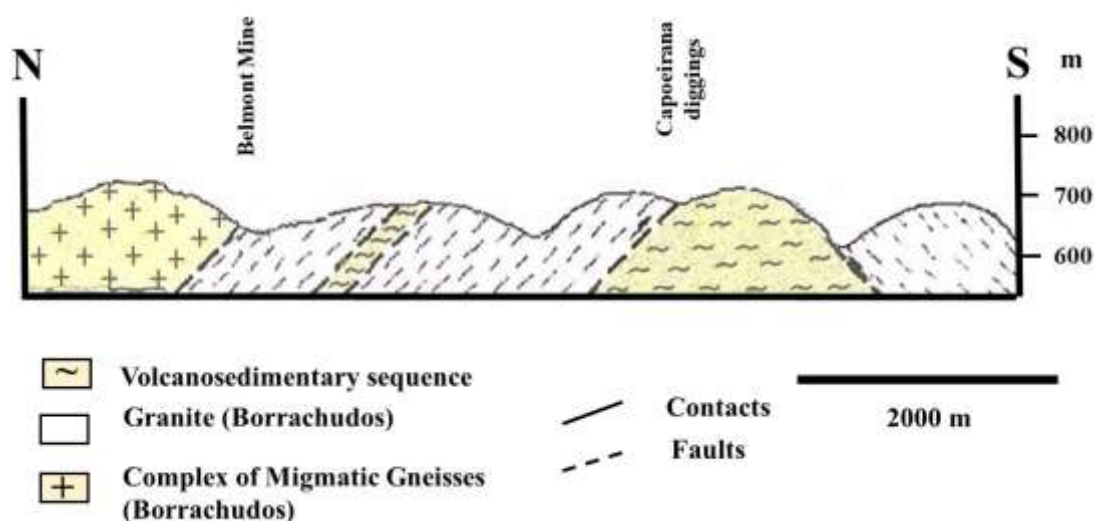
Fig. 2. Geological cross section showing the emerald deposits in the geologic and tectonic environment of the investigated area.
