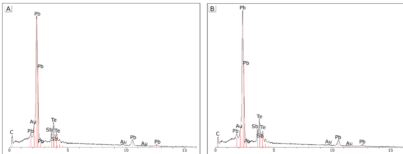
Fig. 4. SEM-EDS spectra of nagyagite from a single lamellae showing chemical composition variation for Pb, Sb, Te and Au. The left spectrum (A) corresponds to nagyagite depleted in Pb, Sb and Te and enriched in Au as compared with the right spectrum (B) that corresponds to nagyagite enriched in Pb, Sb and Te and depleted in Au.
