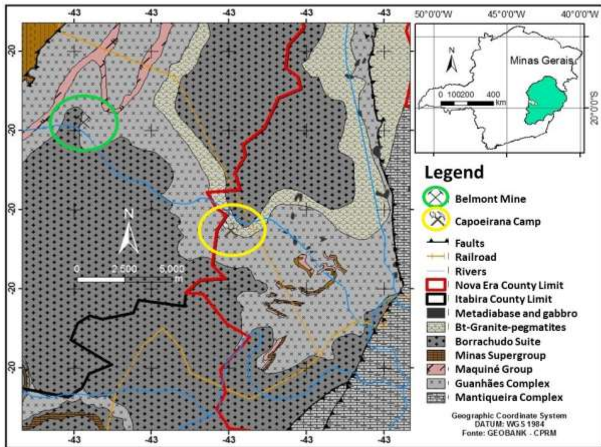
Fig. 1. Geology of the Nova Era-Itabira emerald field showing the location of the investigated deposit (after Horn and Pintea, 2019, modified).
