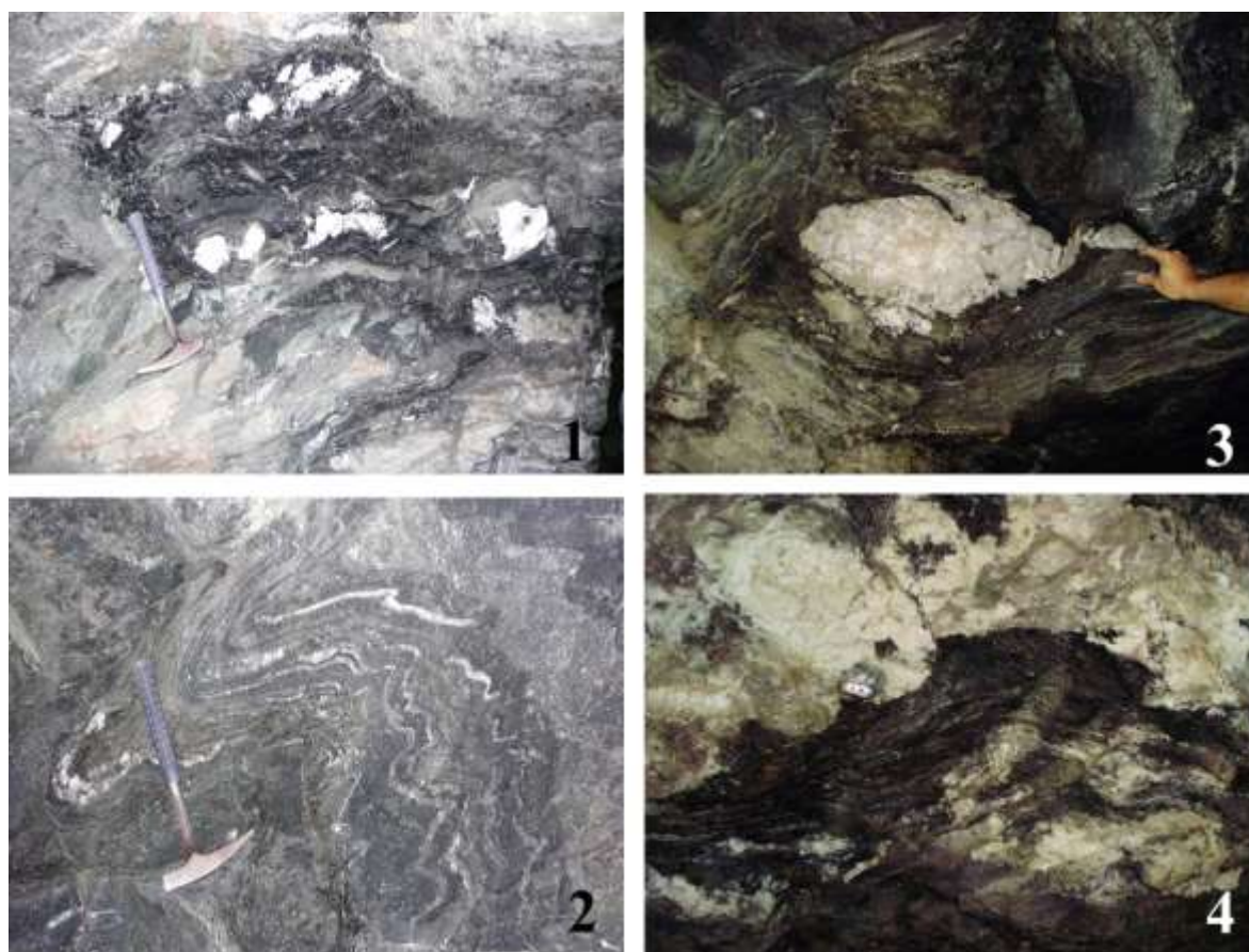
Fig. 3. 1. A concentration of sheared pegmatoid veins cutting the phlogopitite 2. A package of folded rocks. The emeralds are concentrated in the joints of folds; 3. Quartz fish with emeralds in the pressure shadow; 4. Pegmatite vein intercalated with the biotite-phlogopite-quartz schist (Photos: Leal- 1, 2; Horn- 3, 4).
