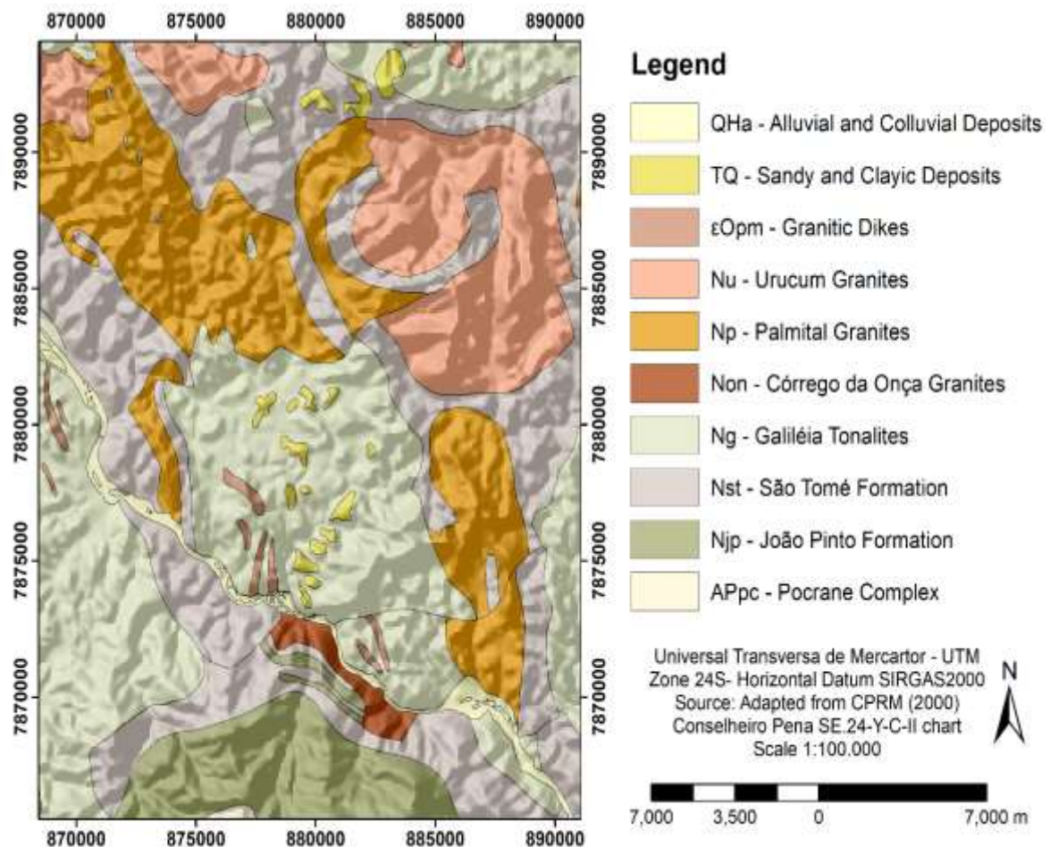
Fig.1. Local geology from the study area. Adapted from CPRM (2000)
