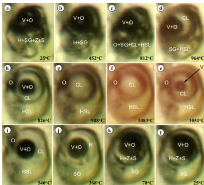
Fig. 4. Melt-melt-fluid immiscibility in remelted silicate glass inclusion from quartz of Bucium Tarnița porphyry Cu-Au \pm Mo deposit; (Metaliferi Mountains, Romania). T_h(\text{CL}) = 1078^\circ\text{C} , X_{\text{NaCl}} = 0.43 , P = 1.6 \text{ kb} , d = 1.0726 \text{ g/ccm} , initial fluid state: V+L. Notations: V-vapor, H- halite, SG- glass, S- another salt, O- opaque, CL-chloride liquid, HSL- hydrosilicate liquid, Z- zeolite-like compound.
