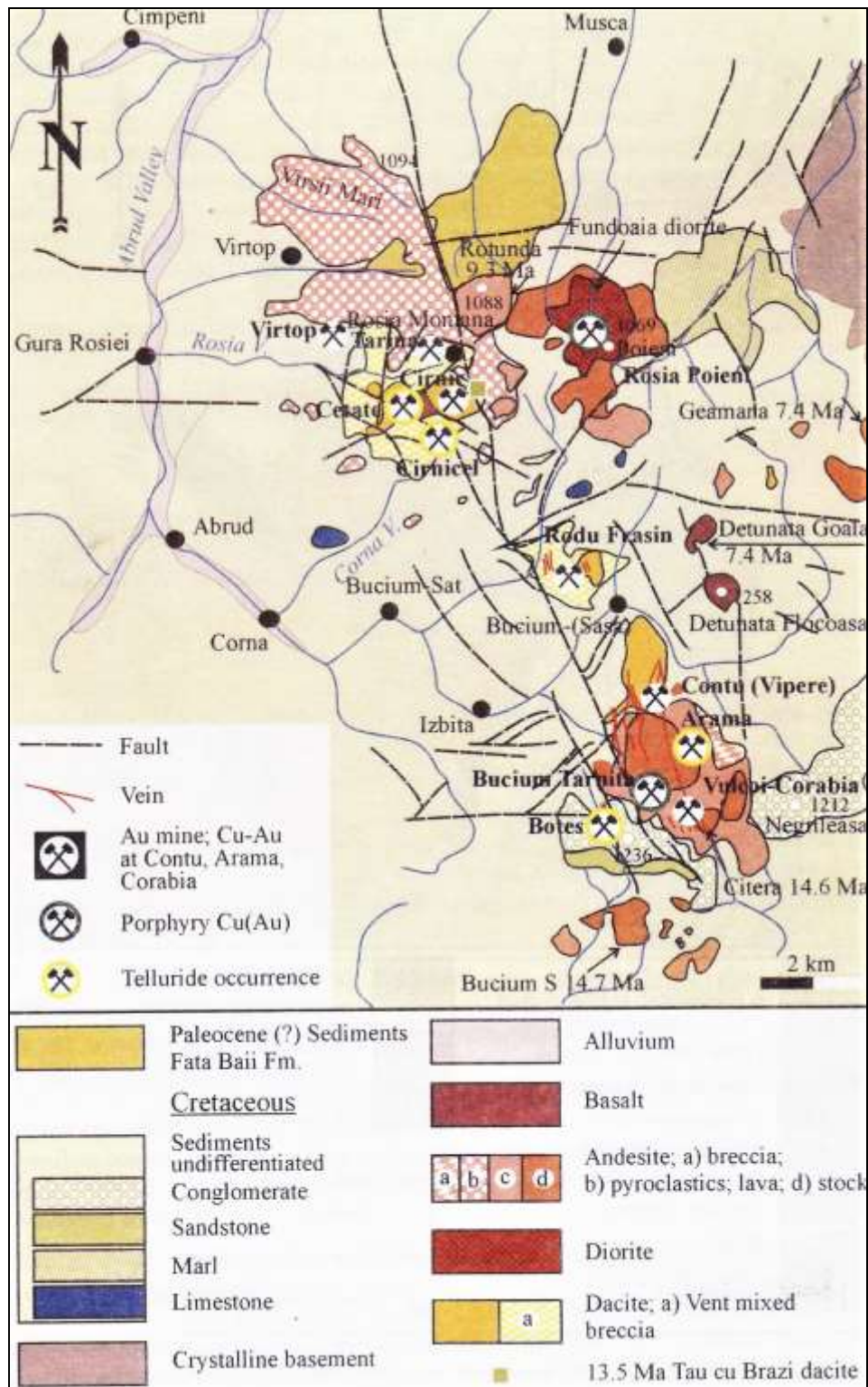
Fig. 1. Sketch map of ore deposits in the Rosia - Bucium area (Ciobanu et al., 2004).
