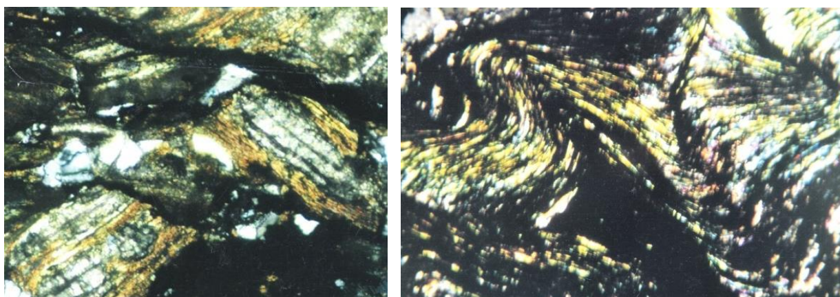
Fig. 2. Carbonatated biotite (yellow relics, cleavage), quartz (white) and graphite (black, veins), TL, N+, x35, (left); Intergrown muscovite (high birefringence, cleavage)/graphite (black), TL, N+, x30, sample BBrc3 (right).
