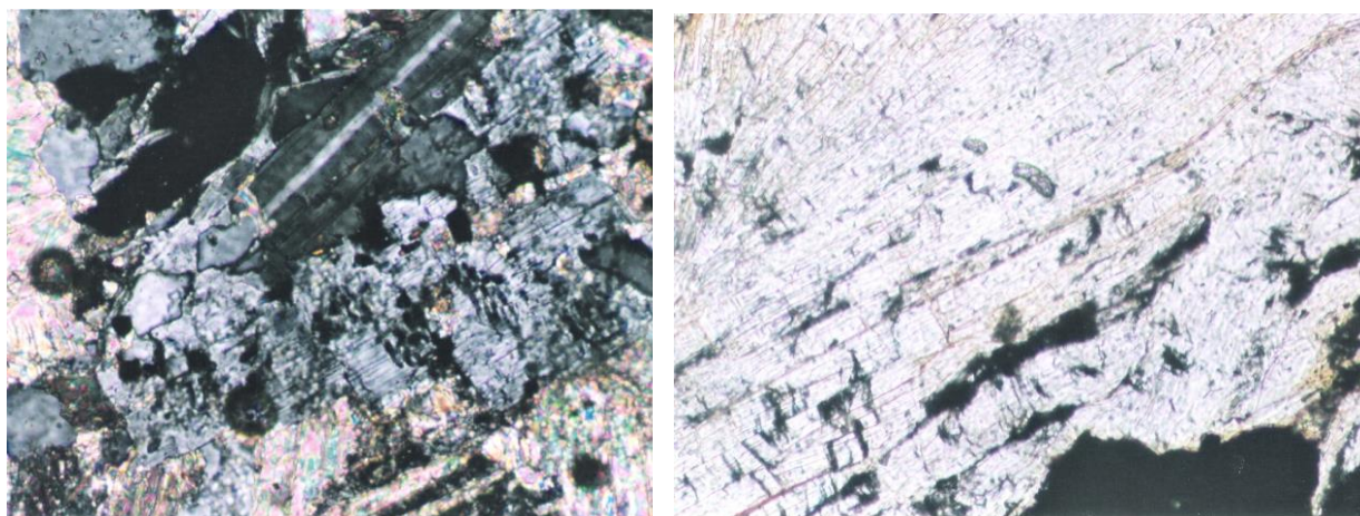
Fig. 8. Coexisting cymrite (grey, perfect cleavage) and celsian (twinned, centre), TL, N+, x30, Barium Belt (left). Cymrite (large crystals, two cleavages) and pyrite (black), TL, NII, x25, Bălan deposit, Sulfide Belt (right).
