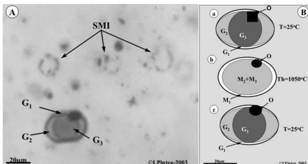
Fig. 12. The complex silicate melt mixture in A , showing 2-3 glass phases at room temperature and during heating procedure in the stage, under the optical microscope the G_2 and G_3 clearly homogenized by fading disappearance of G_3 , as M_2+M_3 in B : in a , silicate rich phase containing the partially melted rounded opaque too, showed in b , at indicated T_h temperature and quenched at room temperature in c . They homogenized by fading vanish of M_3 in M_2 and the process was reproducible, suggesting a critical behavior (?). Probably the complex melt mixture was unmixed “in situ” during decompression or was trapped as immiscible silicate melt phases.
