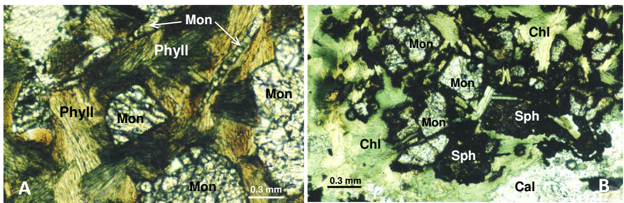
Fig.10. Relics of monazite-(Ce) (Mon) in phlogopite(?) (Phyll, green brown), NII, sample Dt24 (A); Monazite-(Ce) (grey), substituted by sphalerite (Sph, yellow-black), which in its turn is substituted by chlorite (Chl, green), NII, sample D14.
