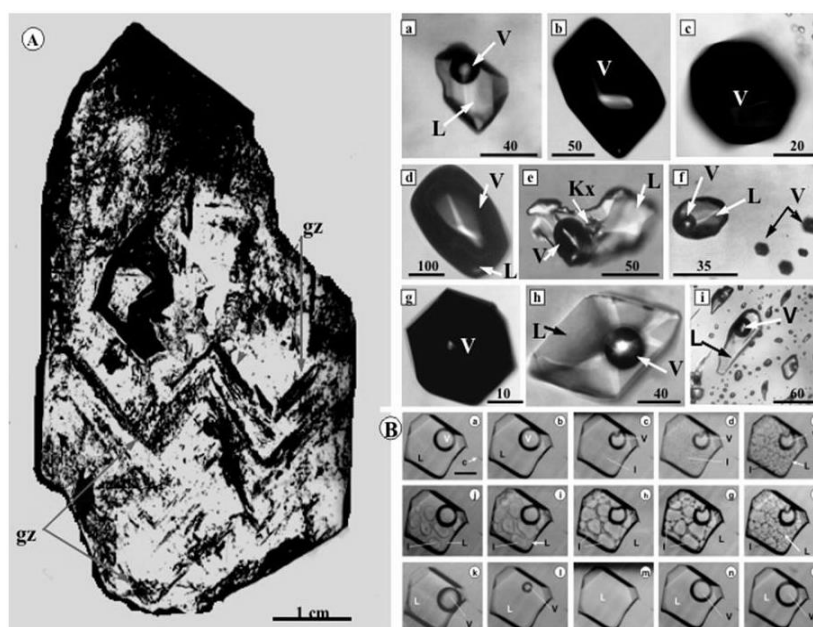
Fig. 9. Typical aqueous fluids trapped in epithermal quartz from Roșia Montană. A. Double terminated prismatic quartz crystal with parallel double zonation (gz). a, h. Primary biphasic fluid inclusion with vapor (V) and liquid (L); b, c, d, g. Isolated vapor-rich inclusions containing a vapor phase (V) and a film of liquid (L); Presumably boiling event recorded by pairs of aqueous- rich (L+V) and vapor- rich (V), trapped in a restricted zone; j. Pseudosecondary biphasic (L+V) assemblage in epithermal quartz. B. Sequences show the complete microthermometric cycle, typical for aqueous-rich inclusions in the epithermal quartz from Roșia Montană, first recorded by Pintea with an original microthermometric stage, working between -196 to +750°C (Pintea et al., 1992): a. and o. +25°C, d. - 40°C (Tf), e. -20.8°C (Te), k. -0.2°C (Tmi), m. +221.5°C (Th), salinity = 0.35 wt% NaCl eq. b, c, f, g, h, i, j, l, n. intermediate temperatures; the fine capillary (c in a. ) had no visible influence on microthermometry; Notations: L- liquid, I-ice, V- vapor; Scale bar in B = 20μm.
