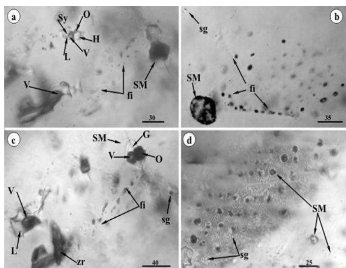
Fig. 7. Secondary hydrosilicate melt and fluid inclusions including brine were formed “in situ” from primary (pseudosecondary) silicate melt inclusions decrepitation during repeated \alpha/\beta transition temperature. a. Multiphase brine inclusions containing halite (H), sylvite (Sy), liquid phase and vapor formed around a decrepitated and altered silicate melt inclusion (SM); b. pseudosecondary trail with vapor-rich fluid inclusions formed by radial microfissure around a decrepitated silicated melt inclusion; c. a zircon microcryst (zr), and silicate melt inclusion decrepitated and released fluid in a radial microfissure system; d. “In-mass” decrepitation of pseudosecondary silicate melt inclusion assemblage produced a continuous cloudy zone of silicate glass globules trail into the surface of microfissure plane. Scale bar in \mu\text{m} .
