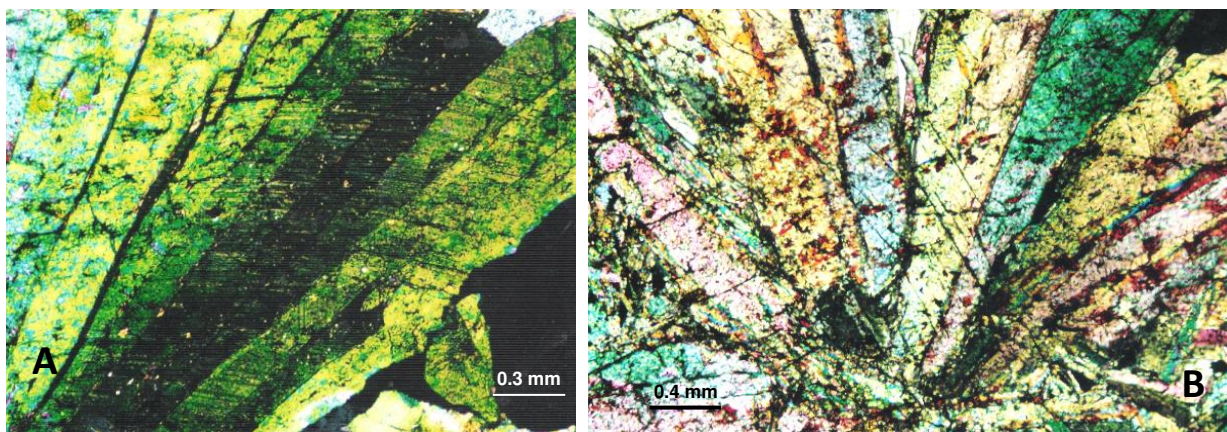
Fig. 6. Monazite-(Ce), thinly twinned on (100), N+, sample Dt6 (A); radial growth of monazite-(Ce), N+, sample Dt5 (B).
