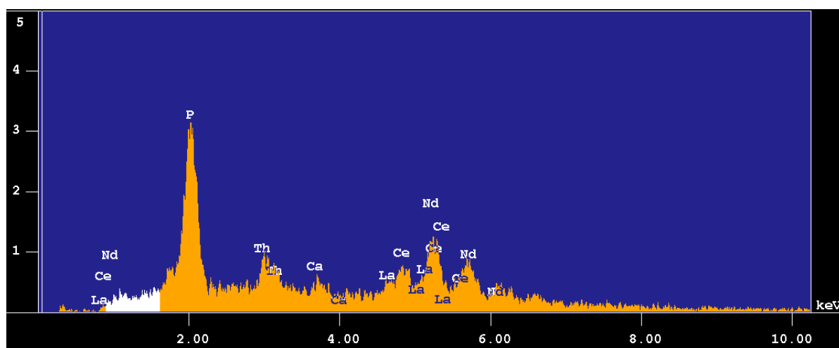
Fig. 16. EDS spectrum of monazite-(Ce) with some brabantite term, sample 7Bel10A.
