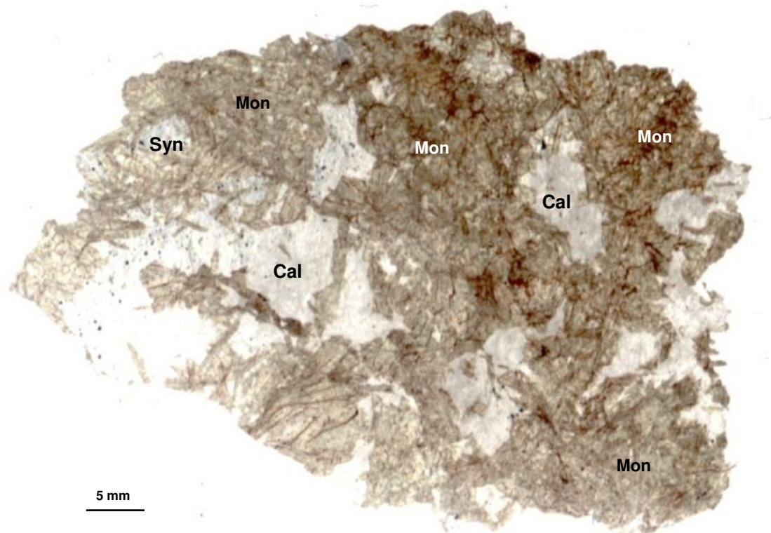
Fig. 4. The scanned image of DT5 polished thin section: monazite-(Ce) (Mon, grey-brownish, partially allanitized), synchysite-(Ce) (Syn, greyish), calcite (Cal, white), Jolotca area. See its optical images in Figs 5A, 5B and 6B.
