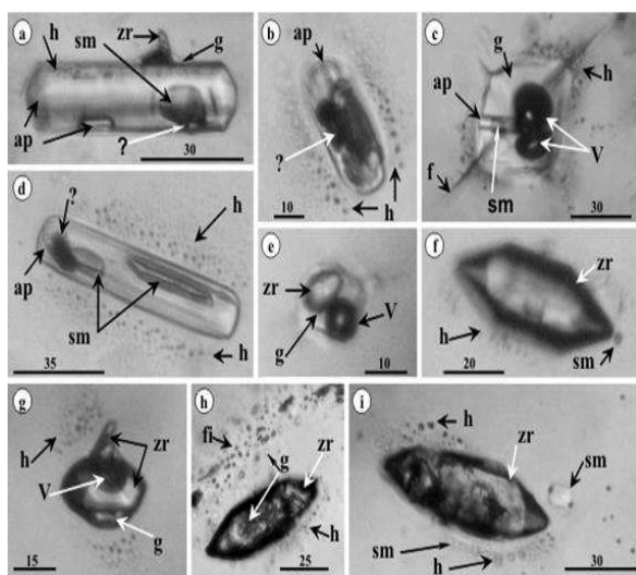
Fig. 8. Hydrosilicate fluid released by successive decrepitation-alteration cycles, inside the \beta -quartz phenocrysts from Roşia Montană. a. Apatite microcryst surrounded by a film of glass (g), agglutinated zircon and another apatite attached needle. A large silicate melt inclusions is also visible (sm,?); b. and d. Decrepitated and altered apatite surrounded by halo formed by silicate glass globules and vapor rich inclusions (the black dots). Undetermined solid inclusions were formed inside the remained apatite, sm- silicate melt inclusion-?. Frequently apatite (c) and zircon (e. and g.) were trapped accidentally and formed multiphase silicate melt inclusions and then decrepitated and altered together, producing silicate melt globules and aqueous fluid in the surrounding “sweat” halos and microfissures (f), g- glass, zr-zircon, ap-apatite, V-vapor, h-halo; f. h. i. The entrapped zircon microcrysts were decrepitated and partially dissolved releasing silicate rich phases and generate “in situ” trails of fluid inclusions in microcracks. Scale bar in \mu\text{m} .
