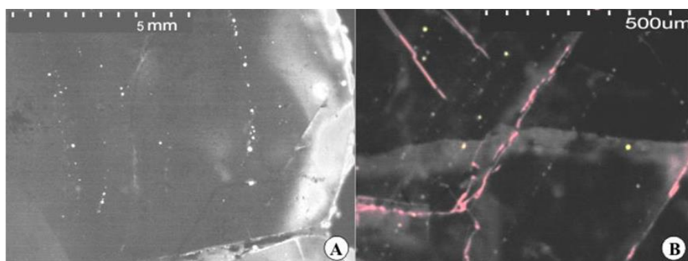
Fig. 5. A. CL image of magmatic quartz shows dark luminescence in the middle and white luminescent rim. High luminescent dots delineated altered silicate melt inclusions, mainly in the resorption layers; B. High magnification of the \beta -quartz internal structure showing yellow luminescent dots of altered silicate melt inclusions, calcite (pinkish-red) and late epithermal quartz (light grey) precipitated into microfissures (modified from Iatan, 2008).
