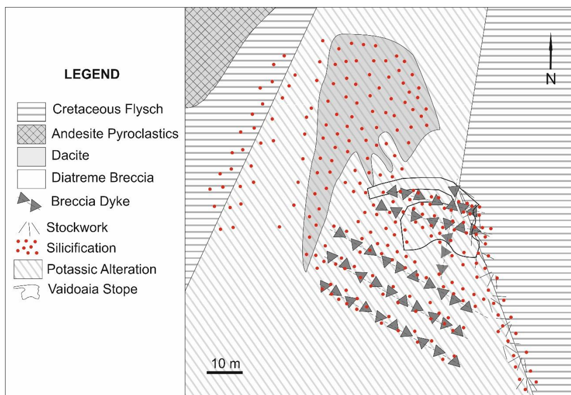
Fig. 4. Surface geology of Văidoaia mining field, provided by Roşia Montană Gold Corporation. The map also shows the distribution of the hydrothermal alterations and the main mineralized structures.
