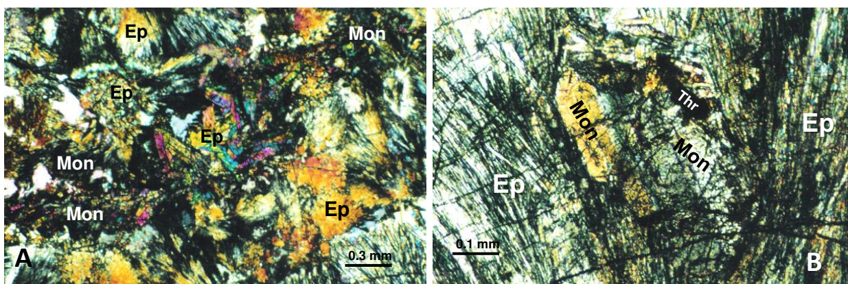
Fig. 7. Monazite-(Ce) (Mon) substituted by REE-rich epidote (Ep) (A); a magnification area from picture A with REE-rich epidote (Ep) grown on twinned monazite-(Ce), N+, sample Dt8 (B).
