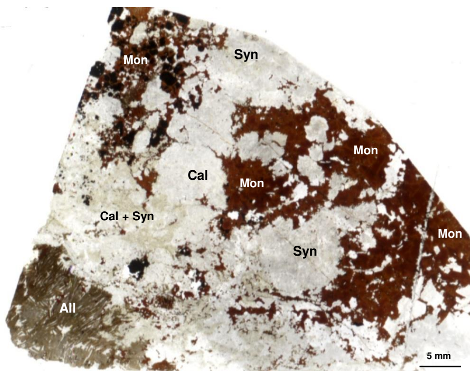
Fig.3. Scanned polished thin section: monazite-(Ce) (Mon, red, right and upper side), allanite-(Ce) (All, acicular crystals, dark brownish-grey, left corner bottom), synchysite-(Ce) (Syn, light grey), calcite (Cal, white, middle), pyrite (black), sample Dt6. See its optical image in Fig. 6A.
