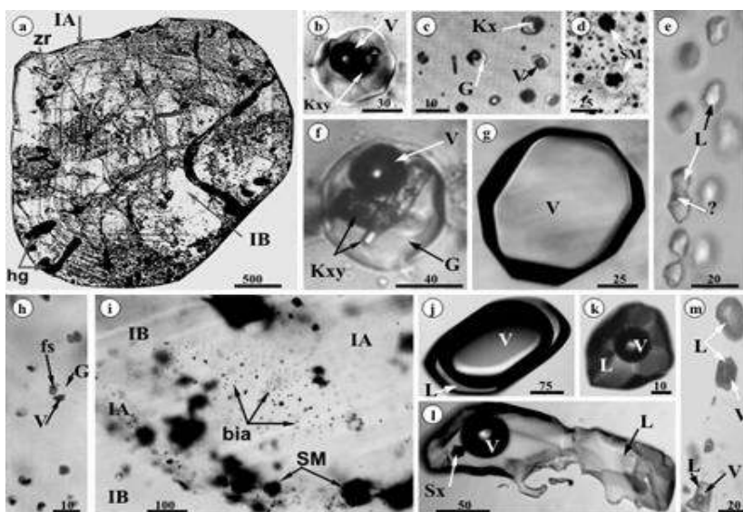
Fig. 3. Silicate melt and fluid inclusions in quartz phenocrysts from Roșia Montană. a. -Transversal double polished thin section on typical \beta -quartz crystal from Roșia Montană dacite showing oscillatory zoned feature of a thin resorption layer- IA and a wide growing zone- IB. Specifically they contain various silicate melt-, fluid inclusions and sometimes embedded solid inclusions as zircon-zr, and hourglass inclusions - hg; b. and f. - Silicate melt inclusions containing glass (G), vapor (V) and daughter solid phases (Kxy); d. - Completely altered silicate melt inclusions with characteristic decrepitation halos formed by secondary fluid inclusions; e. - Monophasic liquid (L) rich inclusion +/- vapor (V) in epithermal quartz; g. Vapor (V) rich inclusion looking empty at room temperature conditions, but during microthermometry a special kind of phase transition were recorded ( see Fig. 3). h. - Brine (fs) trapped in silicate glass inclusions (G-glass, V-vapor); i. - Brine inclusions assemblage (bia) formed “in situ” in a large zone (IB) of \beta -quartz from decrepitated silicate melt inclusions (SM) in a subsequent decompression stage; j. k. - Biphasic vapor – rich and liquid –rich inclusions in epithermal quartz phenocrysts (L-liquid, V-vapor); l. Three phase fluid inclusion in epithermal quartz trapped frequently a liquid (L), vapor (V) and accidentally a solid grain phase of carbonate, silicate or sulfate, but never a real daughter saline (halite) mineral; m. - Biphasic fluid inclusions with variable phase ratios between vapor (V) and liquid (phase) in a secondary trail in magmatic quartz formed “in situ” around decrepitated silicate melt inclusions. Scale bar in \mu\text{m} .
