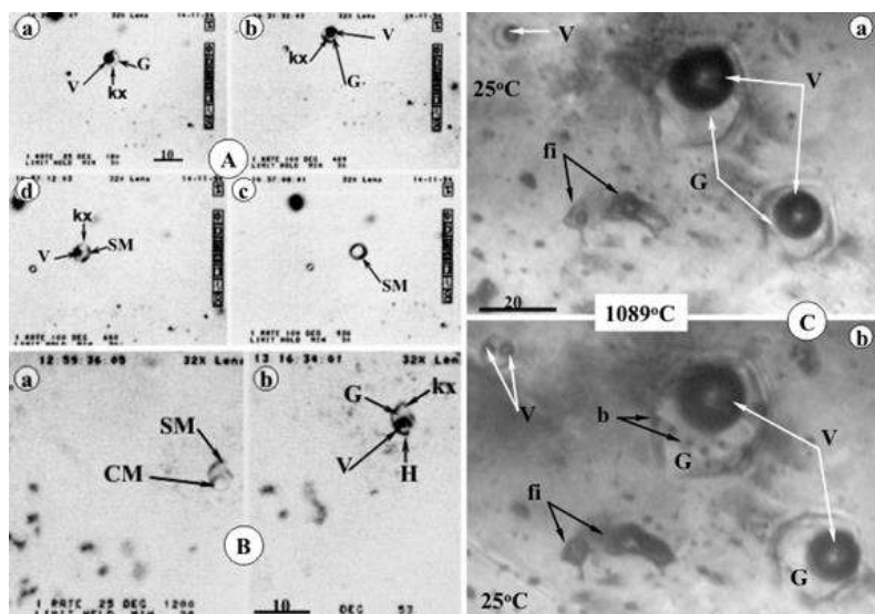
Fig. 13. Silicate melt inclusions microthermometry: A. The smallest silicate melt inclusion selected for homogenization measurements shown at room temperature in a. the coexistence of a vapor bubble (V) and a tiny solid phase (Kx) in the glass matrix (G). During heating in the stage the solid phase melted first above 650°C and the inclusion homogenized by vapor bubble disappearance at 786°C. On further heating above 900°C the silicate melt is in the homogeneous liquid state and do not show any decrepitation feature. Back to the room temperature the cavity contains again the same phase association showed in c. around 600°C, and is still formed by silicate melt (SM) vapor (V) and the growing solid daughter
