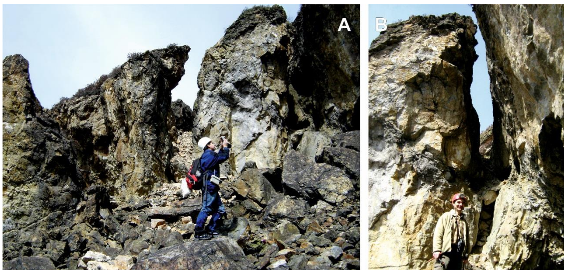
Fig. 13. Old surface extraction works from Văidoaia massif centered on breccia dyke structures: a) the traces of three surface stopes of about 6 m visible depth following three parallel breccia dykes ore bodies from the parallel breccia dyke system occurring in Văidoaia mining field; b) closer view on the south-western surface stope which followed a breccia dyke; the empty space corresponds to the extracted breccia dyke ore body; the mining of all these three breccia dykes continued downwards but the stopes are presently backfilled and no other access is available today from the underground for allowing to estimate the vertical development of the exploitation workings along these ore bodies.
