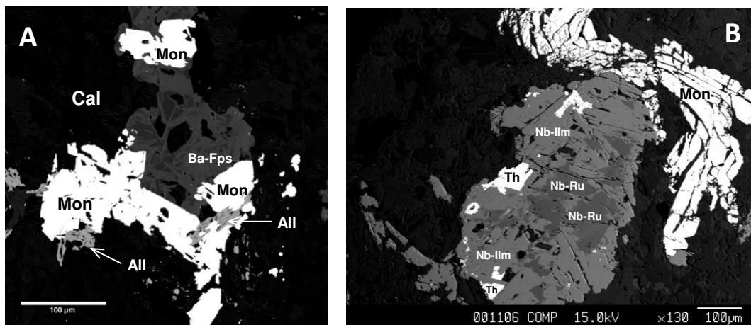
Fig. 13. BSE image of monazite (Mon, white), allanite-(Ce) (All, light grey), Ba-feldspars (Ba-Fps, dark grey with oscillatory composition), calcite (Cal, black), sample 14J1/2 (A); Monazite-(Ce) (Mon, white, top, around niobian ilmenite), niobian ilmenite (Nb-ilmenite), niobian rutile (Nb-Ru, grey dark, relics in Nb-ilmenite) and thorite (Th) on the cracks and cleavage, of Nb-ilmenite, sample Dt 37/1.
