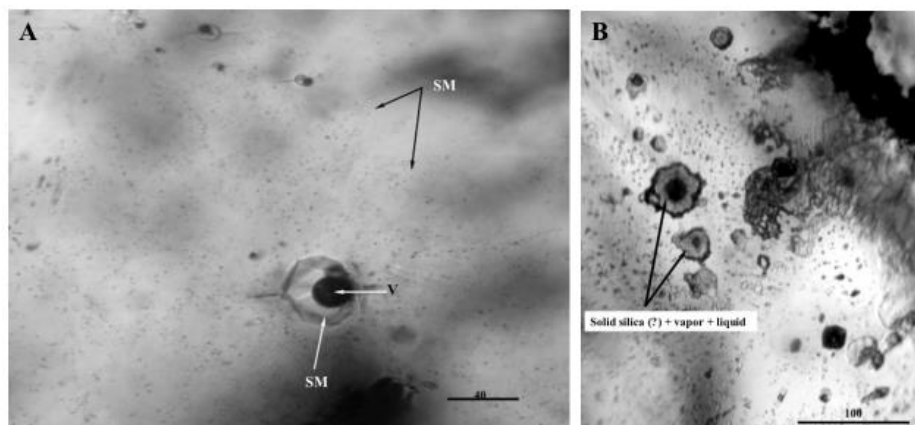
Fig. 15. A. Minute silicate melt inclusions ( < 1\mu to 1-5\mu , i.e. inframineral sized) sprayed around primary silicate melt inclusions in a large growth zone (IB) in the \beta -quartz phenocrysts from Roșia Montană. SM- silicate melts inclusion, V-vapor. Scale bar in \mu m. (see text for more explanation). B. Secondary fluid inclusions in \beta -quartz phenocrysts containing granular silica, vapor bubble and aqueous liquid phase as a thin rim. The hexagonal shape of the inclusions indicates that the microcrack recratized at low temperature. Scale bar in \mu m.
