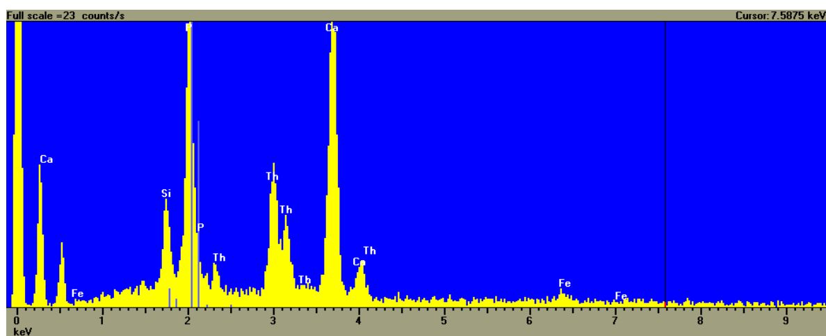
Fig. 15. EDS spectrum of brabantite/huttonite, sample Bel7ce.
