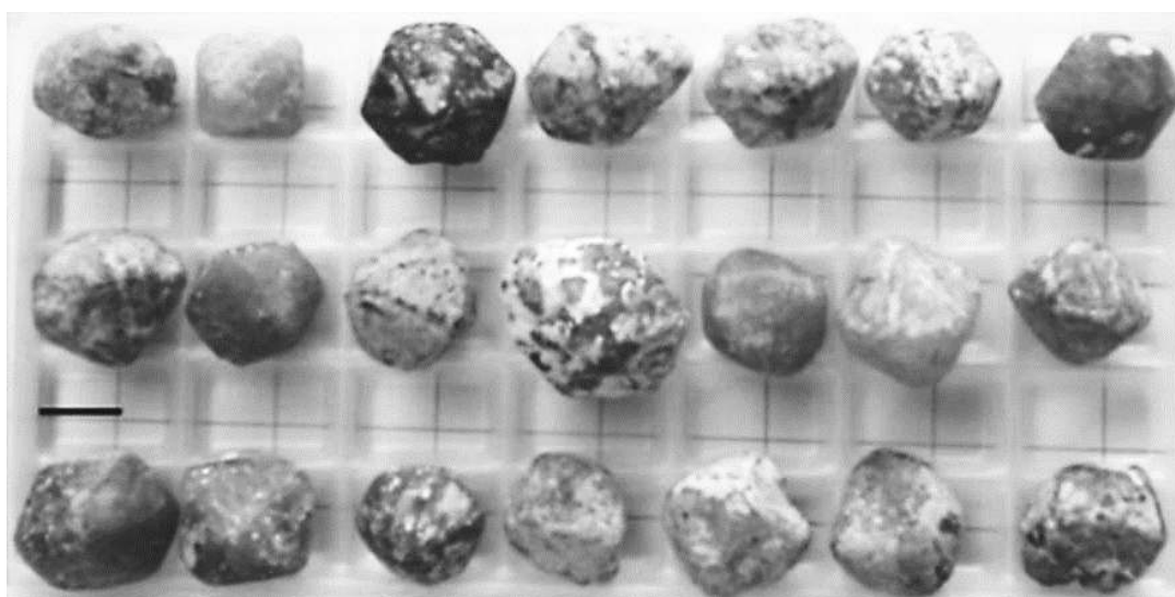
Fig. 2. \beta -Quartz phenocrysts from Roşia Montană dacite. Scale bar 10 mm.
