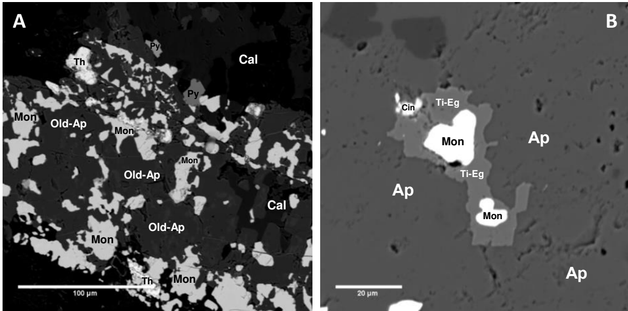
Fig.11. BSE image of the intergrowth/substitution of old apatite (Old-Ap, dark grey) with monazite-(Ce) (Mon, white grey), thorite (Th, white bright), pyrite (Py, grey, top), sample 14J1/4 (A); BSE image of monazite-(Ce) (Mon, two white grains) and cinnabar (Cin, white, small, top) enclosed in Ti-aegirine (Ti-Eg, grey), all in apatite (Ap, dark grey), sample 17J7A/4 (B).
