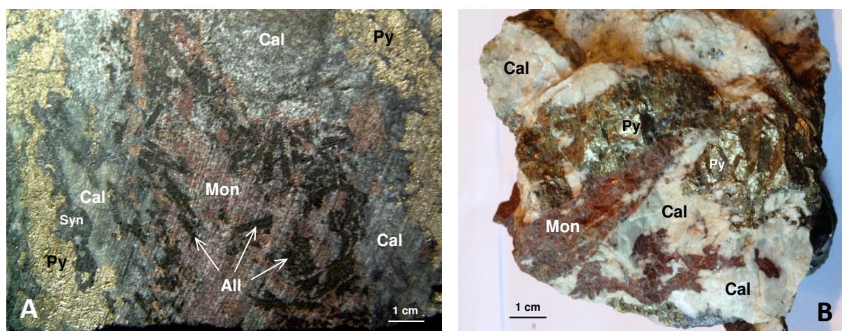
Fig.2. Macroscopical images of primary monazite-(Ce) (Mon, brick red, center) coexisting with primary allanite-(Ce) (All, black prisms), pyrite (Py, yellow), calcite (Cal, grey), synchysite-(Ce) (Syn, dark grey), sample Dt55 (A); Monazite-(Ce) (Mon, red), pyrite (Py, yellow), calcite (cal), sample Dt5c.
