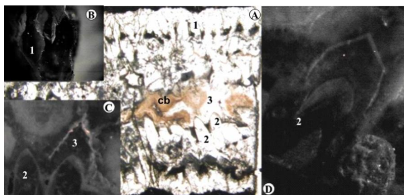
Fig. 6. Different generations of hydrothermal quartz revealed by the CL petrography. A. the quartz vein polished sample; B. Detail of the the first generation of quartz; C. The second and the third quartz generation; D. a close-up view of the second generation of quartz, showing the internal luminescent zonation; (1, 2, 3)- quartz generations, cb-carbonate. Note the irregular surface of the third quartz generation (3) which could be related to a rejuvenation high temperature vapor-rich stage, see text for explanation (modified from Iatan, 2008).
