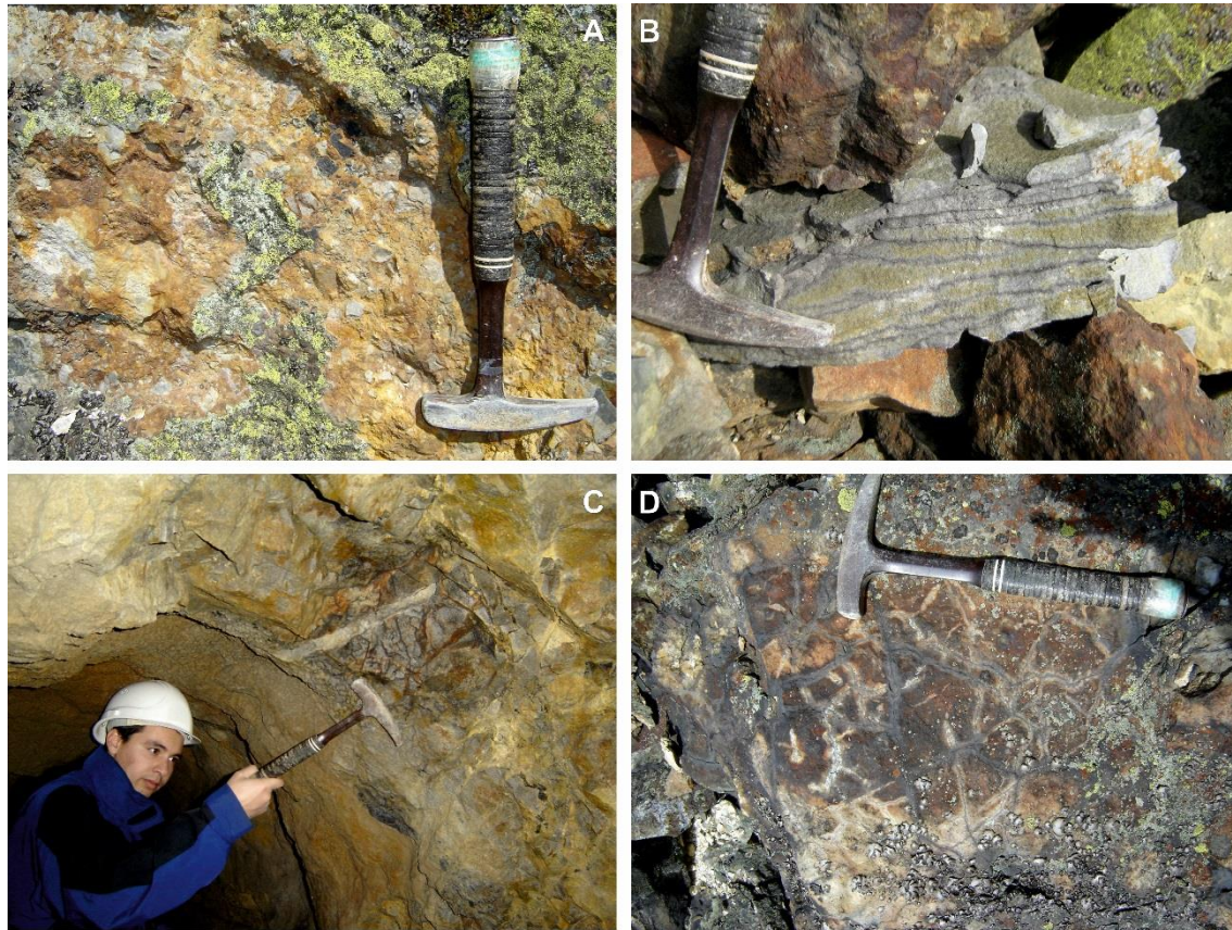
Fig. 10. Outcrop scale mineralizations characteristics: a) typical oxidation pattern developed on vent breccia outcrops due to surface alteration of disseminated pyrite; b) parallel stockwork fissures filled with hydrothermal quartz and pyrite; c) stockwork zone opened in the adit heading west of Coranda Văidoaia - note the trace of the mining drill through the stockwork; d) randomly distributed stockwork fissures within an intense silicified vent breccia.
