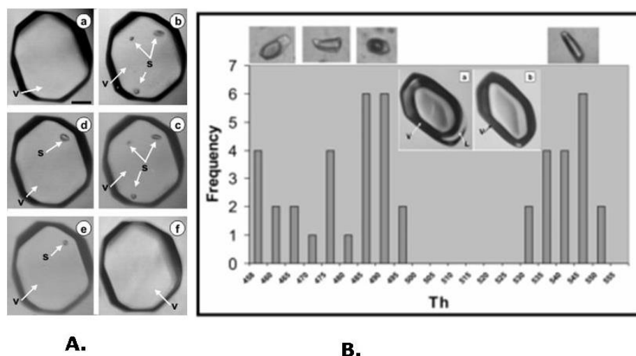
Fig. 14. A. Microthermometric cycle in a vapor-rich inclusion trapped in epithermal quartz. At temperature room condition in a. the microcavity looks like empty but when was cooled down to -170°C, in b. three grains of solid were sublimated (s). The first solid grain melted in c. between -112° and -94°C (H 2 S), d. the second grain melted around -84°C (CH 4 ) and in e. the last grain melted sharply at -56.6°C (CO 2 ), in f. back to room temperature the fluid inclusion contains a presumably pure and invisible gas mixture of CO 2 -CH 4 -H 2 S, no liquid phase was detected by microthermometry in this fluid inclusion type. Scale bar: 30 μm. B. Histogram of vapor homogenization in vapor-rich inclusions from β-quartz in selected fluid inclusions depicted in the upper part of the picture, they were selected based upon their tubular shape. For comparison a vapor-rich inclusion with more regular shape from epithermal quartz is shown at room temperature in a. and close to homogenization temperature around 370°C in b. showing a small unhomogenized white corner down left (modified from Iatan, 2008). Scale bar in A= 30μm.
