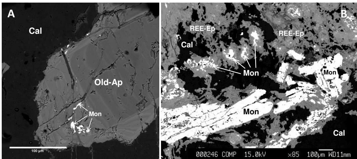
Fig.12. Zoned old apatite (Old-Ap) with Ca variations and with monazite-(Ce) on the cracks, sample 2Bel3 (A); Monazite-Ce (Mon) substituted by REE-rich epidote (REE-Ep, grey, with oscillatory composition), calcite (Cal, black), sample DT2/6 (B).
