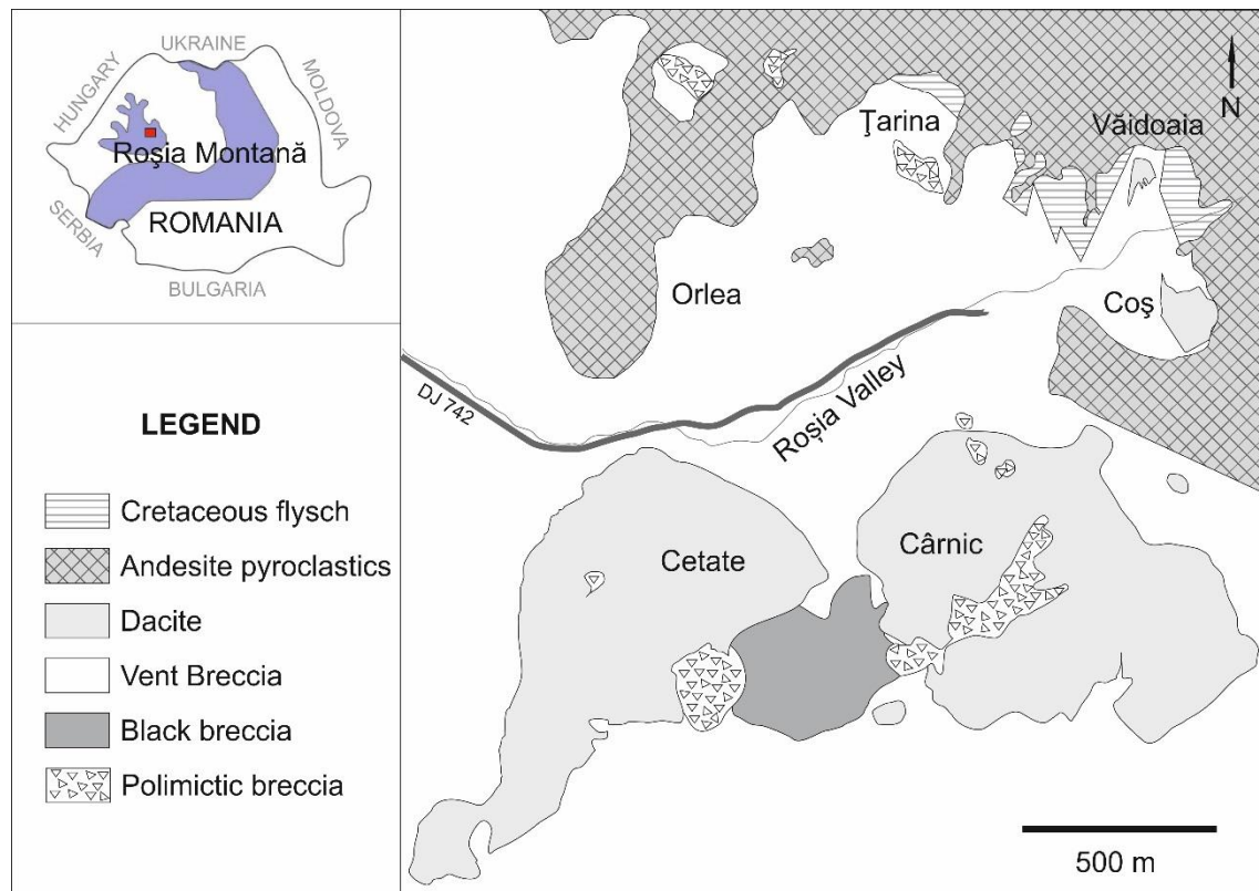
Fig. 1. Geological map of Roșia Montană ore deposit with the main mining fields (Roșia Montană Gold Corporation SRL courtesy). The upper left inset shows the geographic location of Roșia Montană in west-central Romania.
