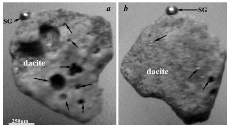
Fig. 10. Globular sulfide (re-melted?) imbedded in dacite-like matrix trapped or attached to \beta -quartz phenocrysts from Roșia Montană. There are many empty vacuoles originally containing the same globules (SG) on the side: a. On the opposite side; b. there are still present tiny sulfide globules incorporated in the spongy rock inclusion (black arrows). Presumably this piece of solid rock was a molten bleb or a remelted mafic rock inside the magma chamber during quartz crystallization (I. Pintea, pers. coll.).
