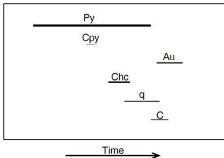
Fig. 15. Paragenetic sequence of the gold mineralization from Văidoaia massif, Roșia Montană including also the emplacement of chinga hydrothermal cement. Abbreviations: Au-gold; Cpy-chalcopyrite; Py-pyrite; C-calcite; q-quartz; Chc- chinga type hydrothermal cement.
