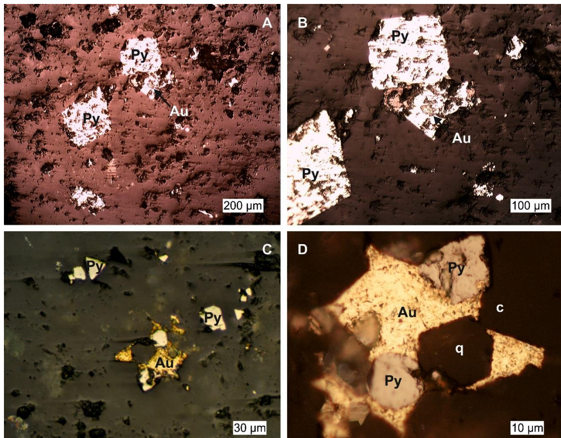
Fig. 14. The ore mineralogy from Văidoaia massif as revealed by polarizing reflected light microscopy (plane polarized light): a) general view of pyrite - gold association from a quartz-adularia II vein; b) detail of the previous image showing gold filling vugs within pyrite; c) general view of the pyrite-gold association from a hydrothermal breccia; d) detail of the previous image showing gold filling the open spaces among various other hydrothermal minerals (pyrite, quartz, calcite). Abbreviations: Au-gold; py-pyrite; q-hydrothermal quartz; c-calcite.
