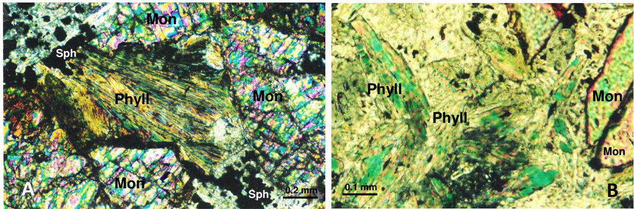
Fig. 9. Monazite-(Ce) (Mon) substituted by phyllosilicates (Phyll), N+, sample Dt24 (A); Monazite-(Ce) (Mon, right side, two prisms) substituted by phyllosilicate/auricalcite (Phyll), N+, sample 5B (B).
