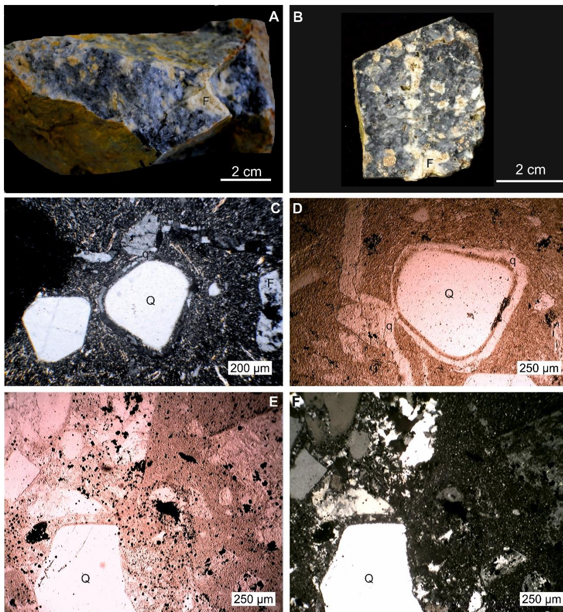
Fig. 7. The dacite from Văidoaia massif: a) hand specimen of porphyritic dacite with dominant feldspar phenocrysts; b) polished slice of dacite showing adularised feldspar phenocrysts set into a silicified groundmass; c) microscopic view in plane polarized light under crossed polarizers of the dacite with rounded to subangular magmatic quartz crystals bordered by a rim of hydrothermal quartz, adularised potassic feldspars and a hydrothermal quartz veinlet; d) microscopic view in plane polarized light of a magmatic quartz phenocryst bordered by a rim of hydrothermal quartz and a hydrothermal quartz veinlet - detail of the Fig. 7c; e) microscopic view in plane polarized light of broken magmatic quartz phenocrysts forming angular fragments; f) Microscopic view in plane polarized light under crossed polarizers of angular to subangular magmatic quartz phenocrysts accompanied by smaller adularised and slightly sericitised feldspar phenocrysts held in a fine grain groundmass. Abbreviations: Q-magmatic quartz; q-hydrothermal quartz; F-adularised feldspars.
