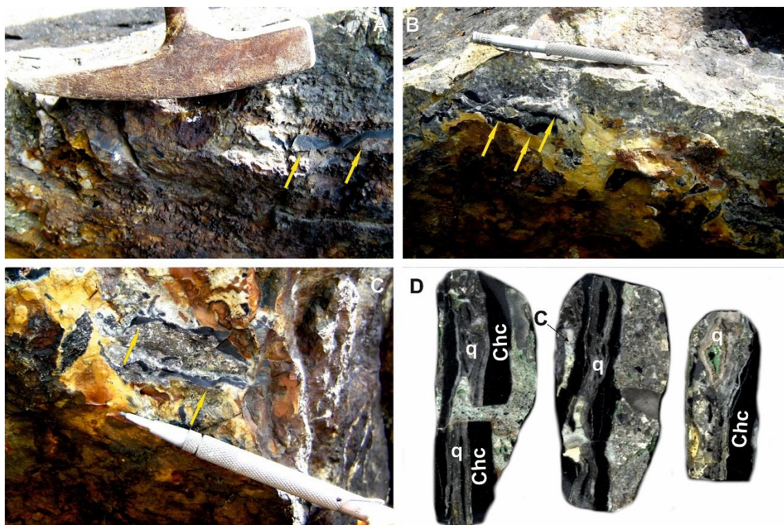
Fig. 11. Macroscopic peculiarities of the veins from Văidoaia mining field: a) individual chinga vein (arrows) crosscutting silicified vent breccia; b) branching chinga vein (arrows) with intense adjoining silicification of the host vent breccia; c) late hydrothermal breccia with chinga clasts and quartz - calcite hydrothermal cement; d) detail of the late hydrothermal brecciation of chinga cement, consolidated with hydrothermal quartz and calcite. Abbreviations: C - calcite; q - hydrothermal quartz; Chc - chinga hydrothermal cement.
