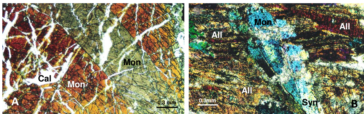
Fig. 8. Largely twinned monazite-(Ce) (Mon) cut by new calcite veinlets (Cal), N+, sample Dt26 (A); Monazite-(Ce) (Mon, middle, like a leaf) relics in allanite-(Ce) and substituted by parisite-(Ce)/synchysite-(Ce) (white spots on monazite), N+, sample Dt8b (B).
