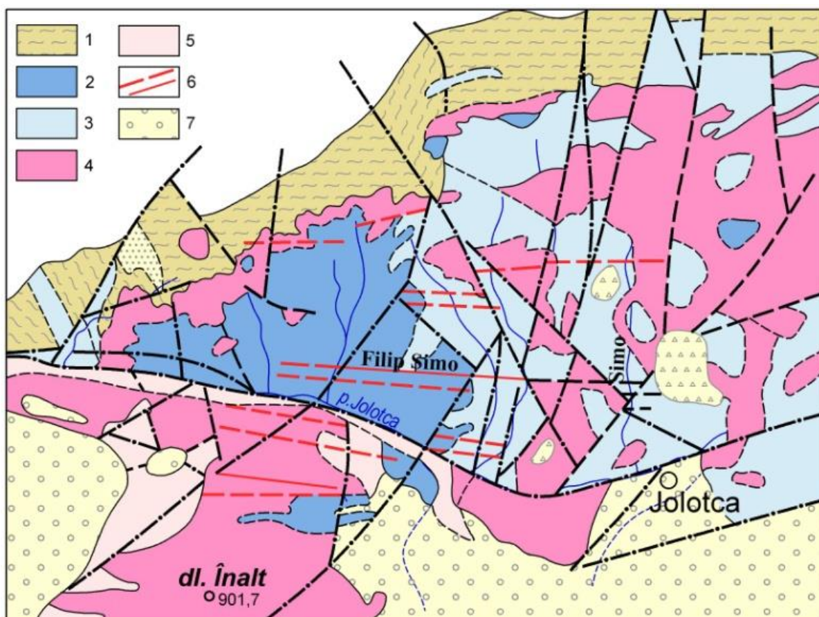
Fig. 1. Jolotca area with mineralized veins field: 1. Metamorphic rocks; 2. Hornblendite; 3. Diorite; 4. Syenite; 5. Monzonite; 6. Veins; 7. Quaternary deposits (Jakab, 2014).
