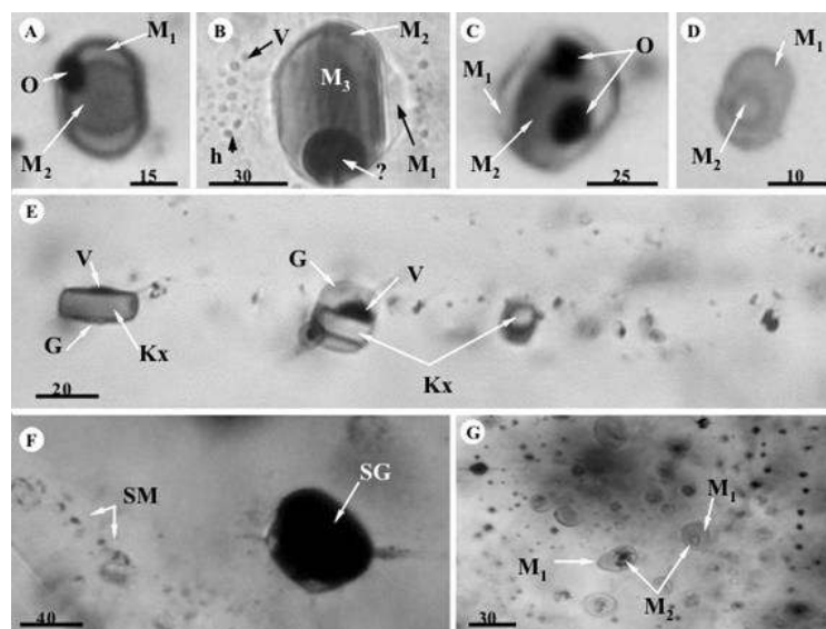
Fig. 4. Possible mafic magma influx trapped as complex silicate melt inclusions in \beta -quartz phenocrysts from Roşia Montană. A. Biphasic silicate glass inclusion contain two different glass phases ( M_1 and M_2 ) and an opaque (see Fig. 12 for microthermometry); B. Complex multiphase silicate glass inclusion with three differentiated glass at room temperature ( M_1 , M_2 and M_3 plus a vapor phase or a spherical opaque-?). This inclusion has been decrepitated after trapping, probably during decompression, showing a characteristic halo formed by separate silicate glass-, and vapor- rich inclusions. It seem that was trapped first as homogeneous mafic melt which then fractionated “in situ” after decrepitation; C, D- The opaque (O) is frequently contained by M_2 phase which is surrounded by fractionated M_1 melt phase; E. Complex crystallized silicate melt inclusions in a trail superimposed on a resorption layer decorated with inhomogeneous silicate glass inclusions showed in Fig. 11, for microthermometry, G-glass, V-vapor, Kx – silicate undetermined (daughter -?) microcrystals; F. globular sulfide (?) included in silicate melt inclusion in a large growth zone close to the resorption layer decorated with silicate melt inclusions (SM); G. Immiscible silicate melts M_1 and M_2 (salt -rich ?) in a pseudosecondary plane. Scale bar in \mu\text{m} .
