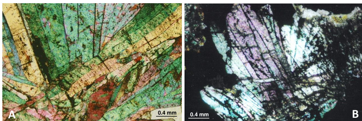
Fig. 5. Optical images of monazite-(Ce) crystals (A and B) from Fig. 4, N+, sample Dt5.
