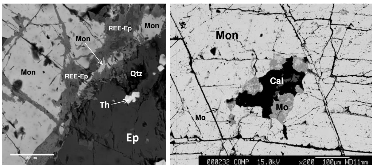
Fig. 14. Monazite-(Ce) (Mon, gray white) substituted by epidote with little Ce and Nd (REE-Ep, oscillatory composition having different grey shades) and with relics of monazite-(Ce), epidote (Ep, dark grey), thorite (Th, light white, small, enclosed in epidote) and quartz (Qtz, black), sample Dt12A/03, point 4 (A); Monazite-(Ce) with molybdenite (Mo) on cleavages and cracks, calcite (Cal, black), sample DT48, point 6 (B).
