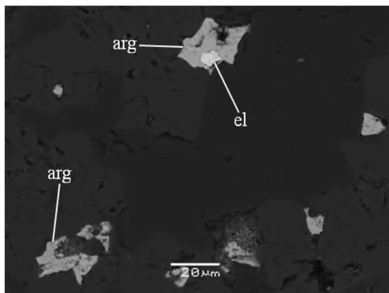
Fig. 3. SEM image of argyrodite - electrum association from a quartz vein overprinting the breccia dyke body exploited within Cârnic 10 Roman network (sample 1660). Abbreviations: arg - argyrodite, el-electrum.
