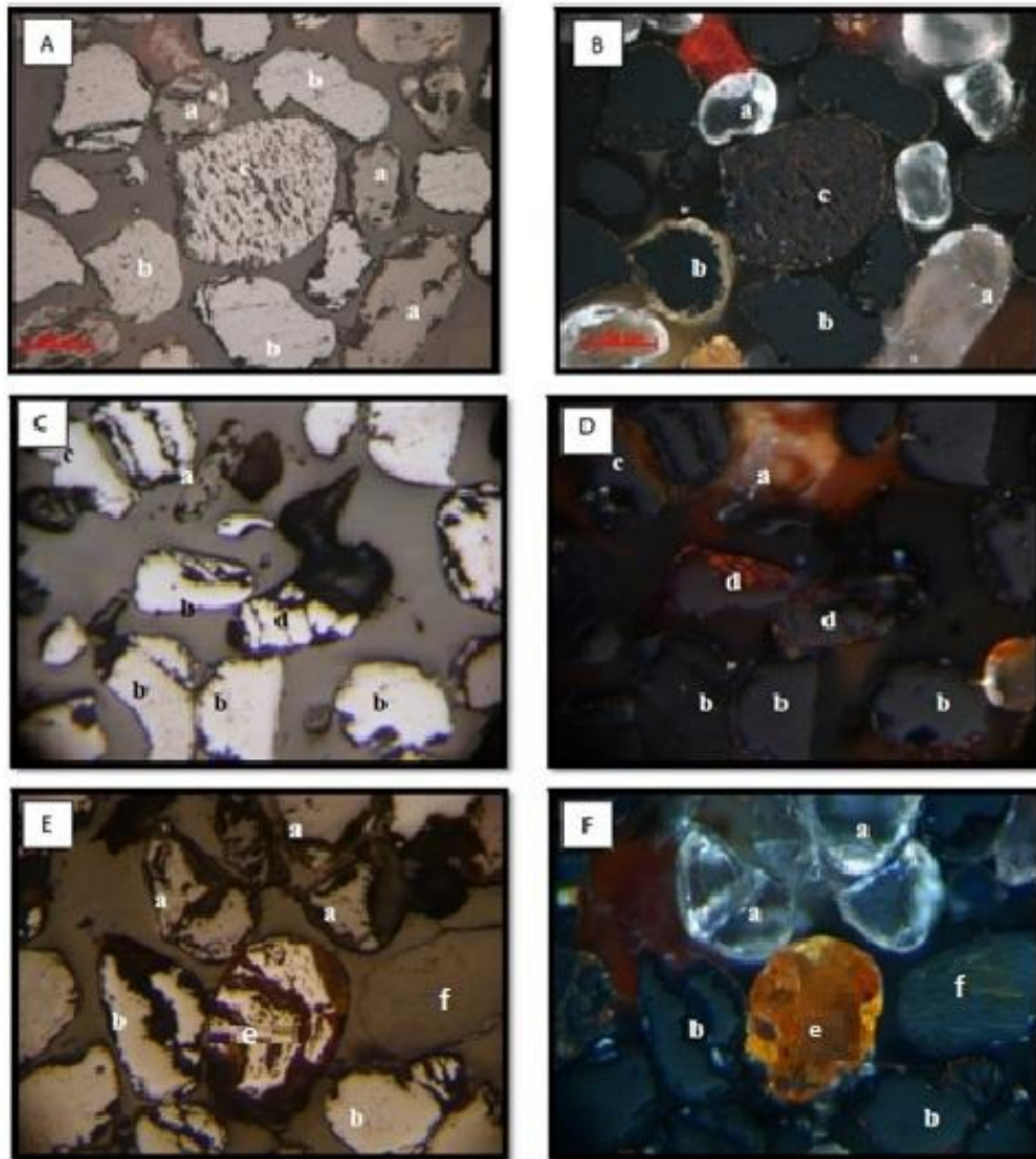
Figure 3: Microscopic views (left column - one polarizer, right column - two polarizers) of the heavy fraction: A and B - zircon, ilmenite, and exsolution of ilmenite within rutile; C and D - zircon, ilmenite, lepidocrocite with internal reflection, and ilmenite with rutile wreaths; E and F zircon, ilmenite, goethite, and hematite. Abbreviations: a - zircon, b - ilmenite, c - exsolution of ilmenite within rutile, d- lepidocrocite with internal reflection, e - goethite, f - hematite.
