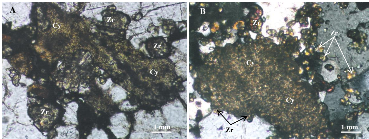
Fig. 1. Rounded, irregular shape of cyrtolite grain (Cy, big grain, yellow-green) with new zircon grains with good shape and high refringence around (Zr), TL, NII, sample G15-1/4 (A); Cyrtolite brown grain aggregate (Cy) with isotropic areas and low birefringence, and new small zircon grains (Zr) around with good shape and high birefringence, TL, N+, sample G15-4/3 (B).
