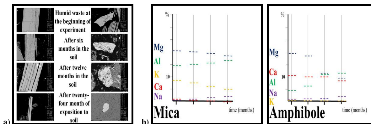
Fig. 5. a. Morphological evolution of the investigated minerals. b. The element evolution in the selected mineral versus time of soil exposure. The slow and continuous liberation of nutrient elements is to observe. Elements like Na and Al are retained in the minerals. For every mineral type 25 grains were investigated and the results treated statistically.
