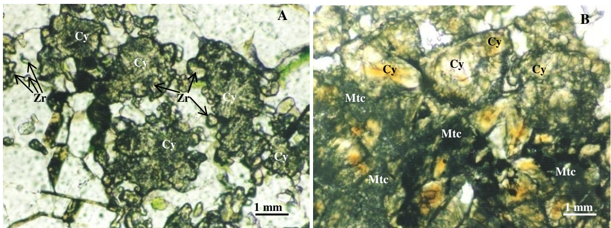
Fig. 2. Fibrous sectorial and marginal zoned of fibrous cyrtolite grains (Cy, green) showing a texture like of that of chiasolite cross, with new generation of small zircon (Zr, clean, no fibrous) grains around, TL, NII, sample G11-2 (A); Fibrous zoned marginal cyrtolite (Cy) with metamict areas (Mtc), with low birefringence TL, N+, sample GM15-1/8 (B).
