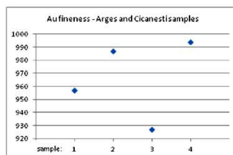
Fig. 2. Au/Ag ratio and the Au fineness of the samples from Argeș and Căcănești.
