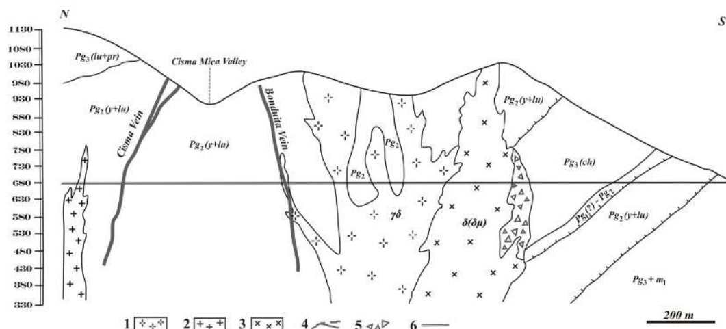
Figure 2. Cross section through the Cisma (Cisma Poiana Botizei) deposit: 1-microgranodiorite porphyries, 2-andesite, 3-quartz-microdiorite porphyries, 4-veins, 5-breccia, 6-gallery, Pg 123 -Poleogene (Eocene) lower, middle and upper.
