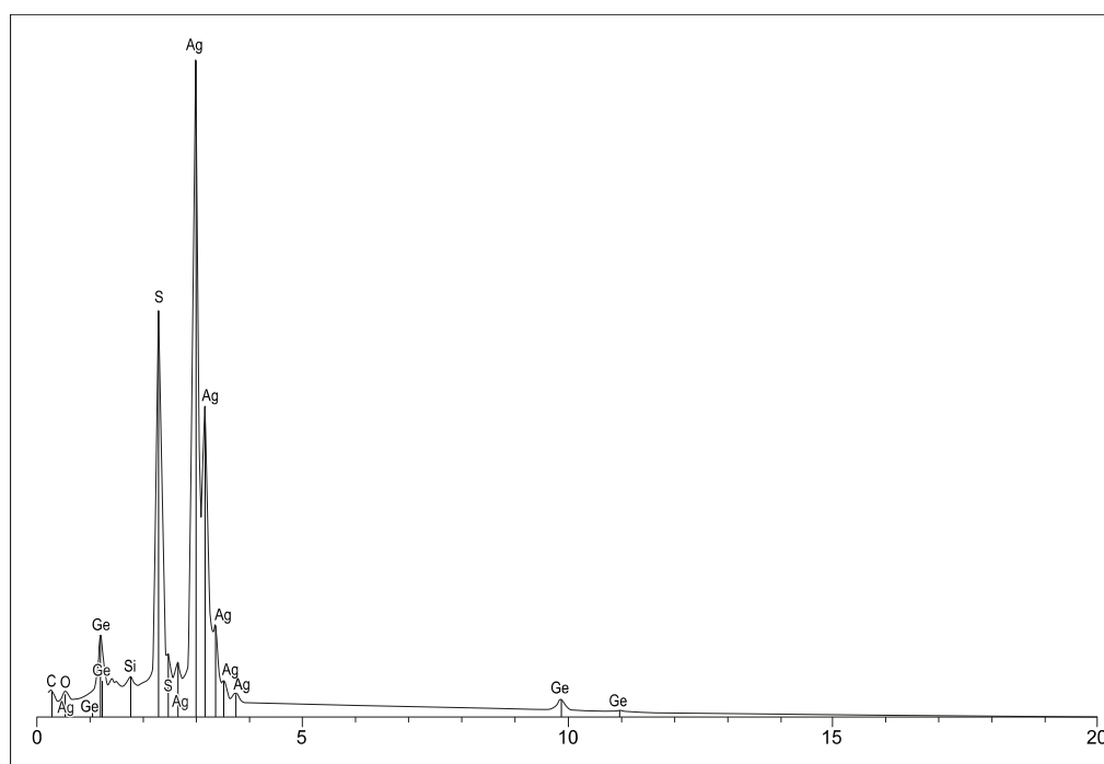
Fig. 4. SEM-EDS spectrum of argyrodite (sample 1572), showing the peaks of the chemical elements defining this mineral: Ag, S, Ge.
