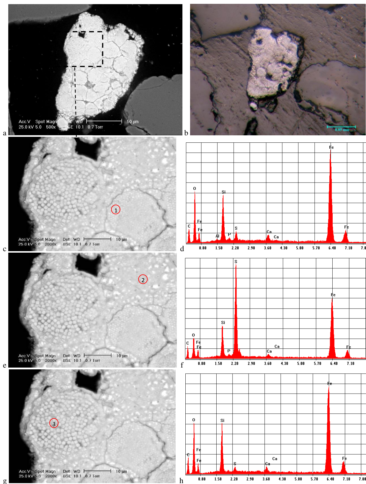
Figure 2: Microscopic images of the analyzed sample (P4) in polished section: a – on electronic microscope (SEM); b – on chalcographic microscope (N//); c, e, g – detail showing the analyzed spot; d, f, h – diagrams presenting the results detailed in Table 1
