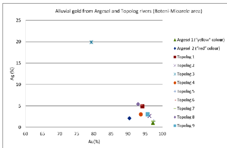
Fig. 3. Au/Ag ratio and the Au fineness of the samples from Argeşel and Topolog.
