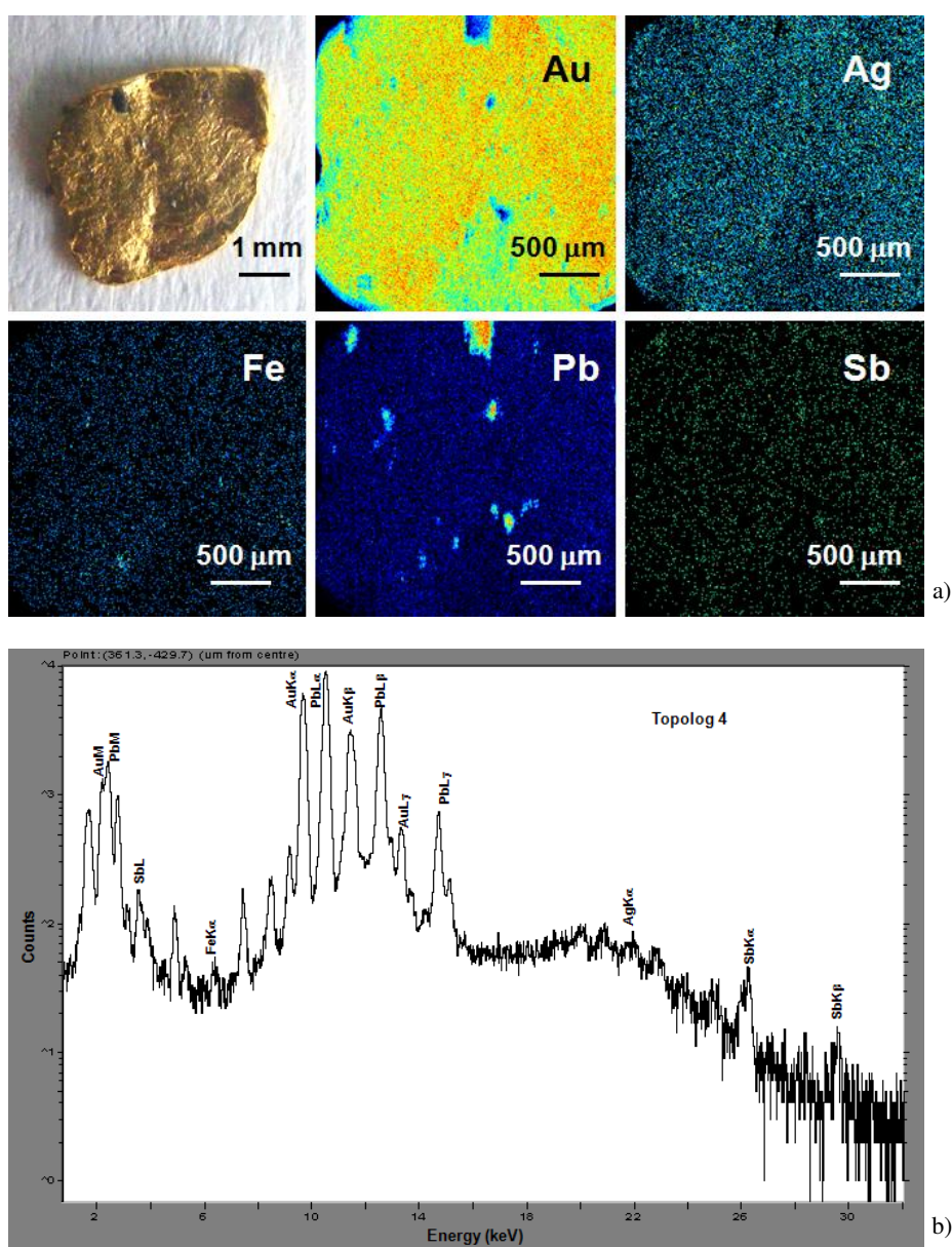
Fig. 4. Topolog 4 sample - micro-PIXE elemental maps (a) and point spectrum - Pb (b).
