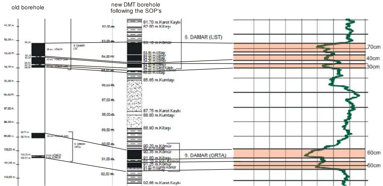
Fig. 2: Correlation between old borehole and a new borehole and a geophysical borehole measurement; example from the Thracian Basin near Malkara.
