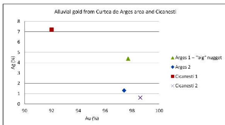
Fig. 2. Au/Ag ratio and the Au fineness of the samples from Argeș and Căcănești.
