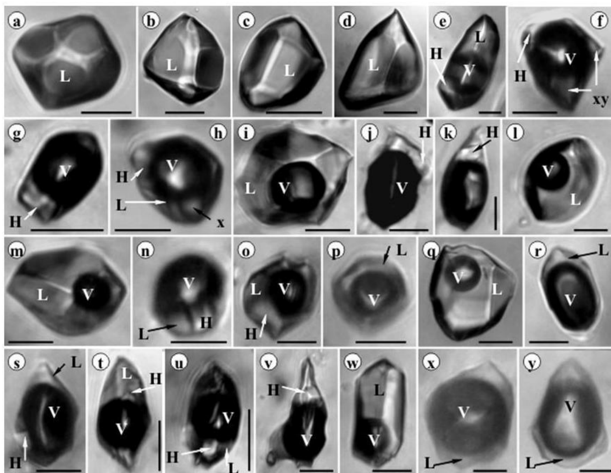
Figure 3. Liquid monophase-, (a, b, c, d) – biphasic-, (i, l, m, p, q, r, w, x, y) and triphase-, (e, f, g, h, j, k, n, o, s, t, u, v) fluid inclusions in barite nodules from the bentonitic Valea Chioarului mining prospect (geol. V. Todoran, 1997 - sample courtesy). Notations: L-liquid, H- halite, V- vapour. Homogenization temperature in un-stretched biphasic fluid inclusions ranged between 154° and 240°C (n = 30). Rarely, triphase fluid inclusions (n=4) showed Th= 263-330°C, with estimated salinity of 30-34 wt% NaCl eq., and formation pressure between 28 and 96 bars. Scale bars: 10 µm.
