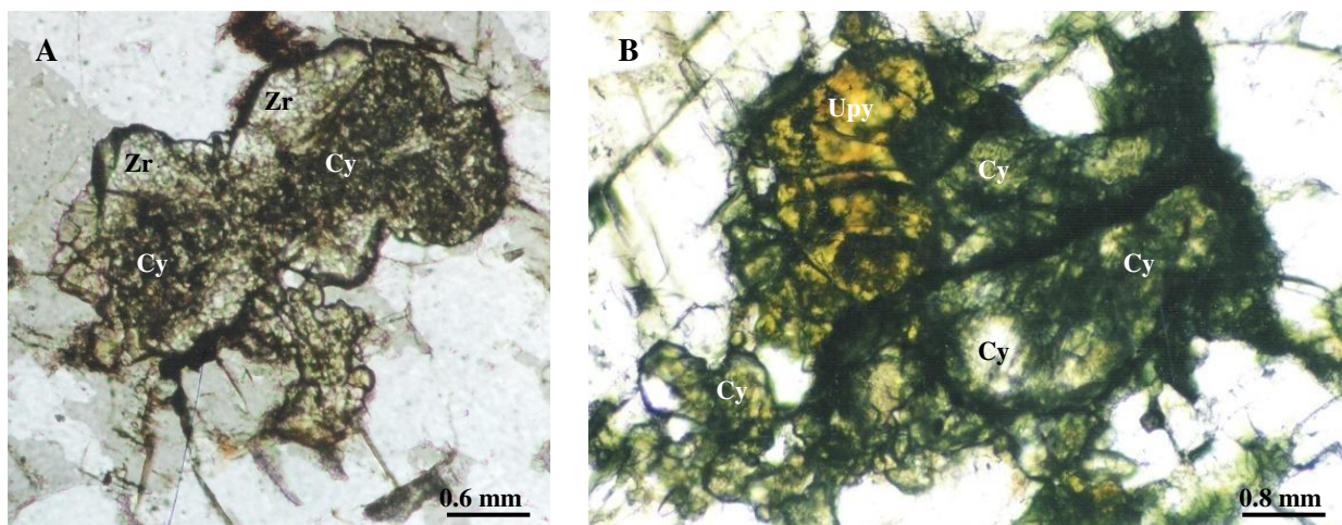
Fig 7. Zoned crystal:cyrtolite (Cy, core, high Hf), zircon (Zr, rim, clean, no Hf), sample GM31 (A); uranpyrochlore (Upy, yellow orange) associated with green radioactive cyrtolite variety (Cy), LT, NII, sample G15-1 (B).
