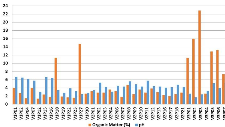
Fig. 2: The pH values versus organic matter. The lowest pH values have highest organic matter concentration.
