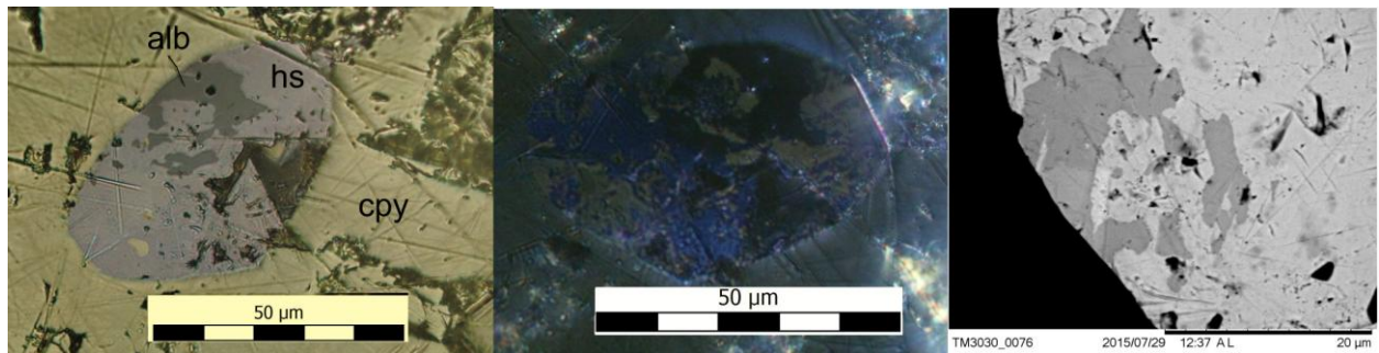
Fig. 4. Albunite (alb - isotropic) intergrown with hessite (hs - birefractive, anisotropic) also possibly containing stützite, in a subhedral inclusion in chalcopyrite (cpy). Left – plane-polarized reflected light, oil immersion; centre – the same grain under crossed polarizers, rotated position; right – BSE image of a detail containing the albunite grains.
