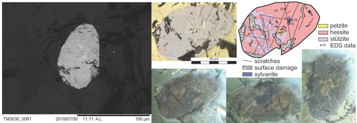
Fig. 3. Composite hessite – stützite inclusion containing minor sylvanite and petzite. Left – BSE image; upper row right – reflected light microphotograph of the same grain in oil immersion, and sketch showing the mineral composition and location of the EDS analyses; lower row left – reflected light microphotographs of the same grain rotated at different angles, in oil immersion and crossed polarizers
