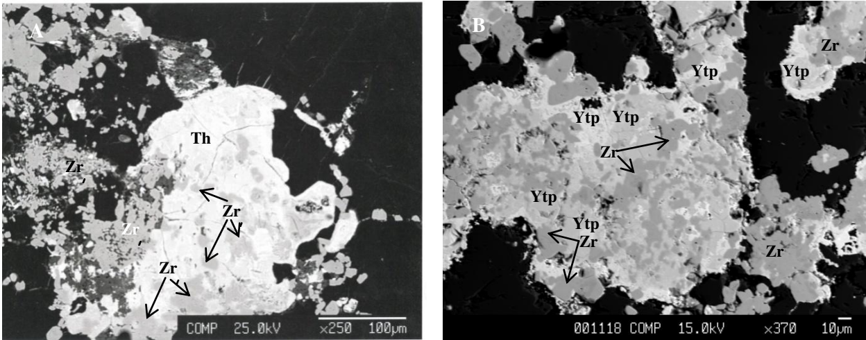
Fig. 4. BSE image of oscillatory composition in thorite (Th): white more Th, Nb, Y, Fe and white grey with more Si and Th and less Nb, Fe and Y, many zircons (Zr) inside and around, sample G11-5/2a (A); BSE image of zircons (Zr) enclosed in yttrpyrochlore-(Y) (Ytp) with oscillatory composition: more Ta and less Y (white grey) and more Nb and Y (white), sample G15BA/1 (B).
