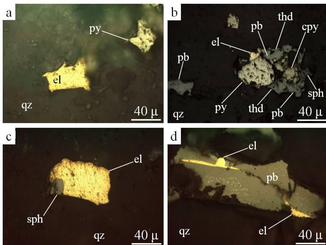
Fig. 1. Microscopic view (polished sections, plane polarized light) of the mineralogical association from the ore body mined out in Cărnic 10 Roman network (breccia dyke and overprinting quartz veins), Cărnic massif, Roșia Montană: a - electrum and pyrite in quartz gangue; b - electrum, polybasite, tetrahedrite, chalcopyrite, sphalerite and pyrite; c - electrum covering sphalerite; d - electrum crosscutting and deposited on polybasite. Abbreviations: cpy - chalcopyrite; el - electrum; pb - polybasite; py - pyrite; sph - sphalerite; thd - tetrahedrite; qz - quartz.
