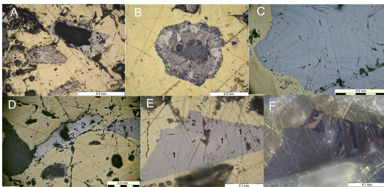
Fig. 1. Reflected light microphotographs of assemblages in chalcopryrite-dominated vein filling. A: Concentric pyrite-fahlore intergrowth (centre-left) and fahlore (1) replaced by enargite (2) in chalcopryrite aggregates; B: Concentric fahlore – enargite – quartz pseudo-inclusion in chalcopryrite, C: Recurrently zoned fahlore, structural attack with Ar ion beam. D: Composite pseudoinclusions containing fahlore (1) stützite (2) and sylvanite (3). E: Fahlore (1) engulfed, corroded and replaced by enargite (2). F: the same image under crossed polarizer, displaying the anisotropy of enargite and the fahlore rounded relics inside it.
