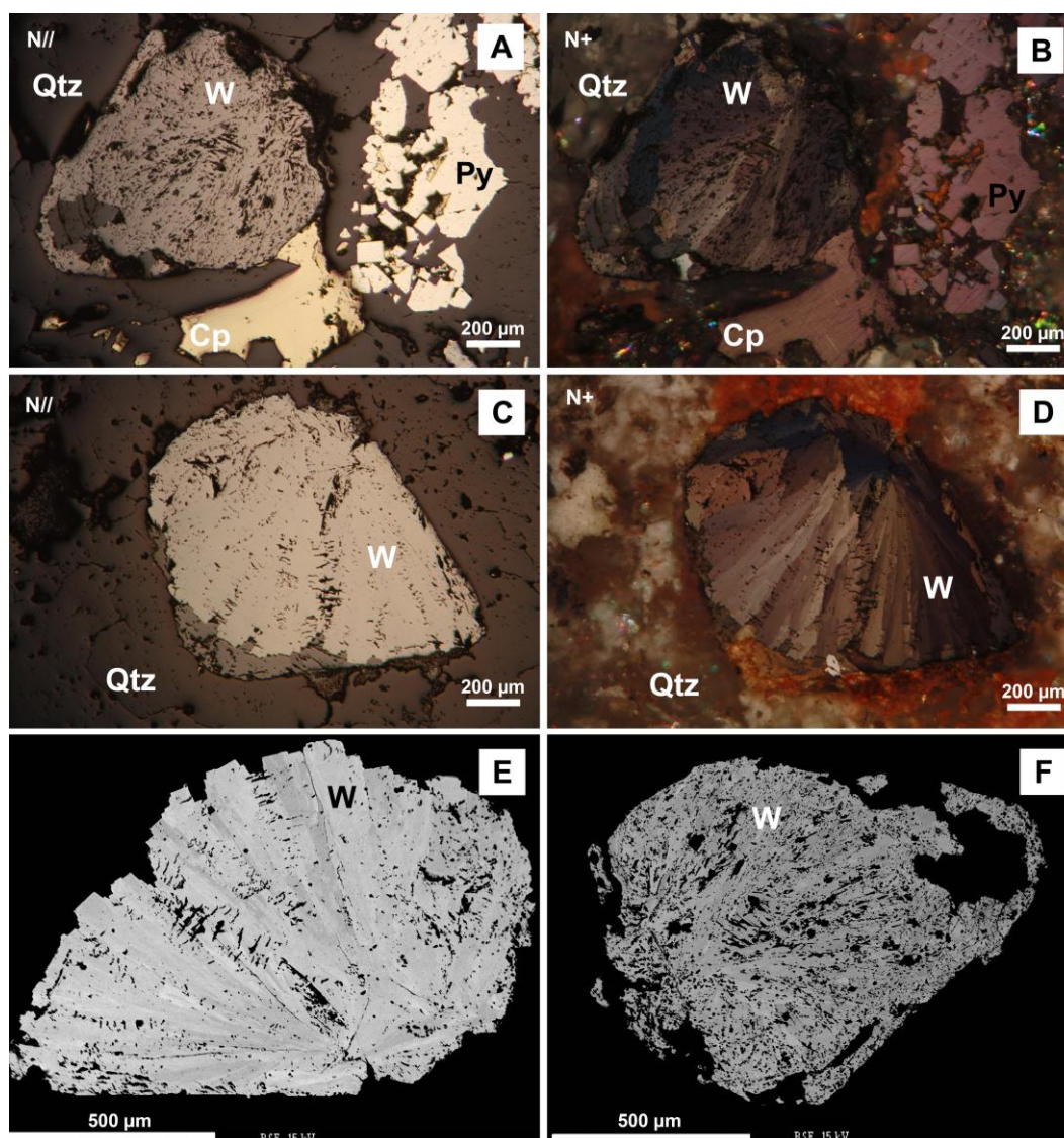
Figure 3. Wolframite (ferberite): A-wolframite associated with pyrite, chalcopyrite included in quartz parallel nicols, B same image as A, cross nicols, C-wolframite included in quartz, D-same image as C, cross nicols, E and F - Backscattered electron images (BSE) of wolframite.
