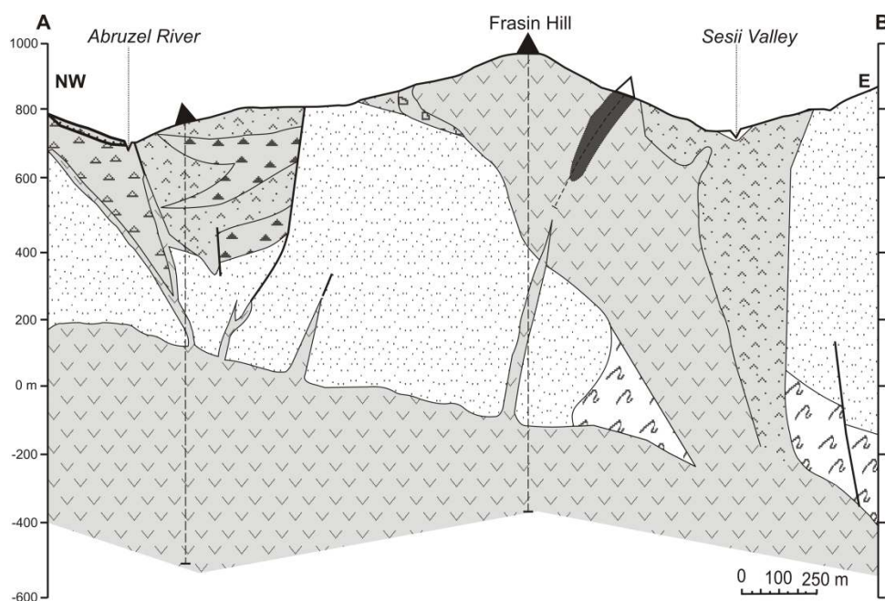
Fig. 2. Cross-section through Bucium Rodu-Frasin area (compiled using the drill core data from R.M.G.C., I.P.E.G., and authors' unpublished data). For legend, please see Fig. 1.
