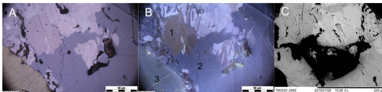
Fig. 2. Stützite-sylvanite composite pseudoinclusion in chalcopryrite. A: Plane polarized reflected light, oil immersion. B: Crossed polars, oil immersion, 1- sylvanite, 2-stützite, 3- chalcopryrite. C: BSE image
