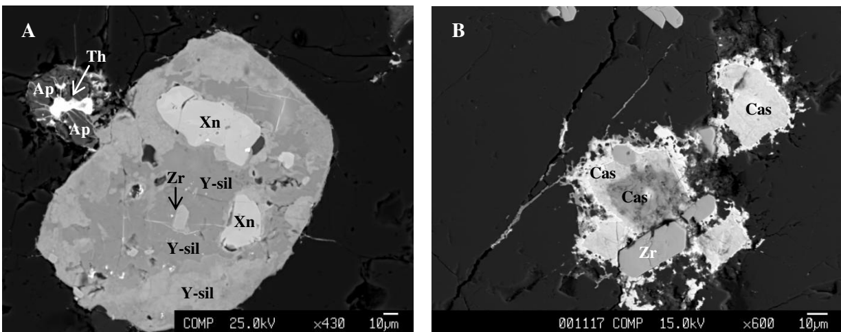
Fig. 6. BSE image of Y-silicate grain (Y-sil, prism, with oscillatory composition), with zircon (Zr) and xenotime (Xn) inside; in the corner up left thorite with zirconium (Th) with apatite (Ap) around, sample GM31/10, (A); BSE image of zoned cassiterite (white, grey white) with enclosed zircon (prismatic, grey), sample G11-4A/1, (B).
