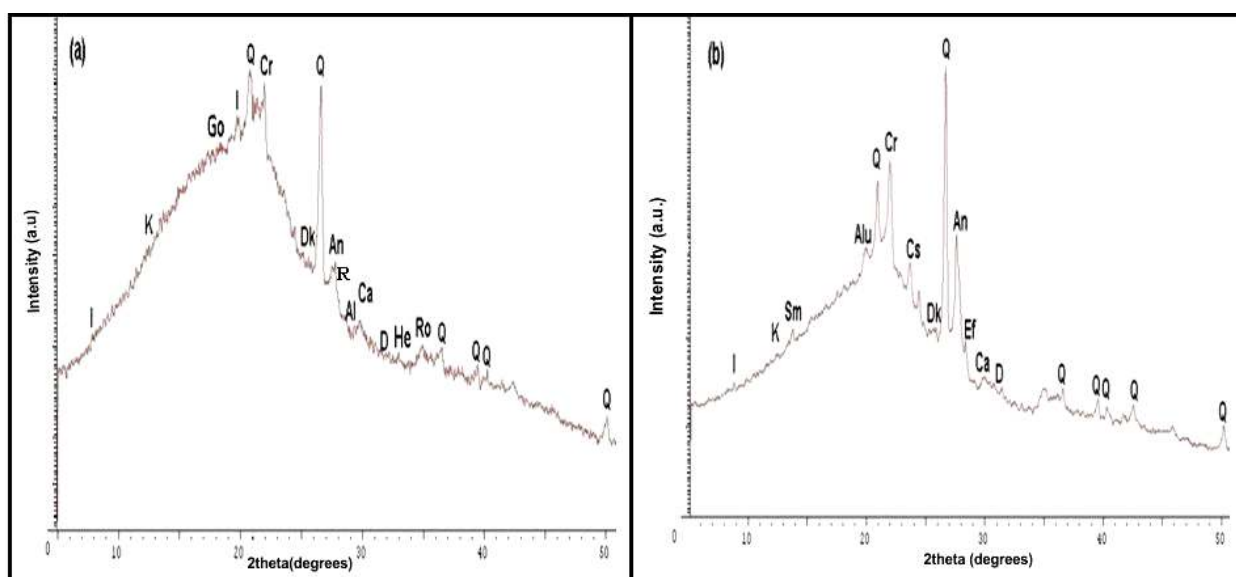
Fig. 2. XRD diffractograms of the peat samples (where Q=quartz, Cr=cristobalite, I=illite, K=kaolinite, Dk=dickite, An=anorthite, Al=albite, Ca=calcite, D=dolomite, Cs=calcosiderite, Ef=efremovite, Sm=simonellite, Ro=rorsite, Alu=alunogene, He=hematite, Go=goethite, R=rutile)
