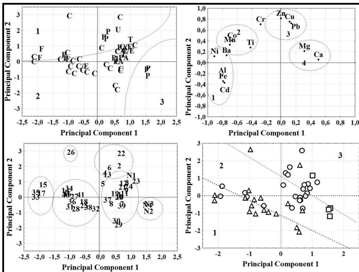
Fig. 2. Results from the Principal Component Analysis (PCA) of the samples of sediments from water bodies in the Caparaó National Park: a. for anthropogenic activity (C: coffee; C/E: coffee/eucalyptus F: fish farming; P: preserved; PA: pasture; U: urban, T: tourism); b. for elements; c. for the sampling points; c. for geographic location (triangle: western flank; quadrangle: central part; circle: east flank).
