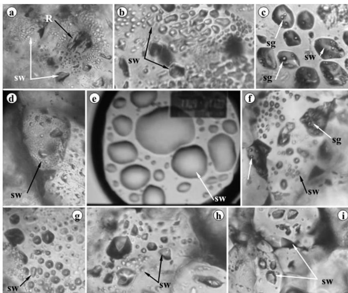
Figure 2. Presumed former supercritical water droplets (liquid cluster assemblage) trapped in the coarse grain quartz from Metaliferi Mountains (a. Larga – DI Roatei ; b. Talagiu; c, d, f, g, h, i – Deva) analogous to the supercritical water shoved in diamond anvil cell experiment under critical pressure (Mibe, 2001; 2010- http://www.youtube.com/kenmibe ). R- solid restite, sw- liquid (vapour) water, sg- silica globules. Not to scale.
