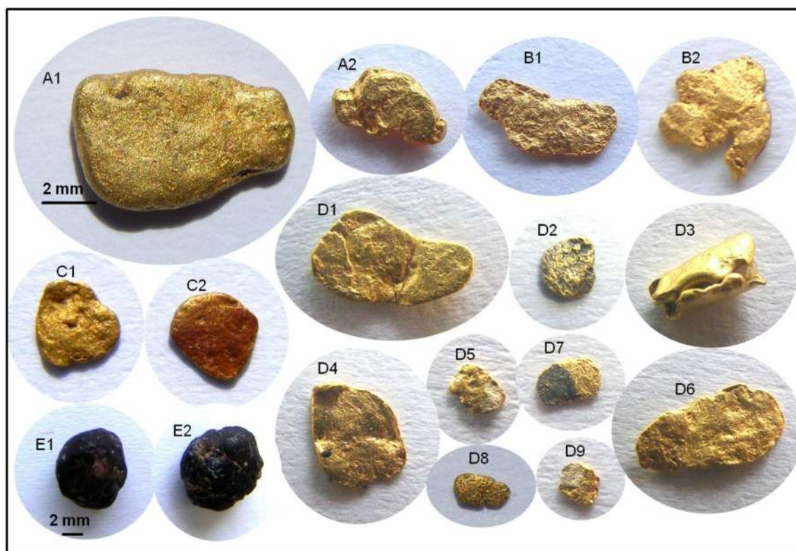
Fig. 1. Alluvial gold grains (nuggets) from Argeș (A1-A2), Căcănești (B1-B2), Argeșel (C1-C2) and Topolog rivers (D1-D9) and the polygonal dark colored grains from Căcănești (E1-E2).
