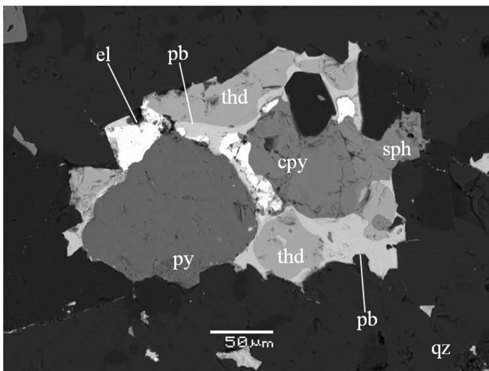
Fig. 2. SEM image of the mineral association consisting of electrum, Ag minerals and common sulfides from the ore body exploited within Cârnic 10 Roman network. The image represents a detail of Fig. 1b. Abbreviations: cpy - chalcopyrite; el - electrum; pb - polybasite; py - pyrite; sph - sphalerite; thd - tetrahedrite; qz - quartz.
