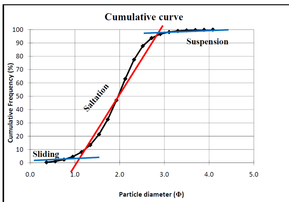
Figure 4: The cumulative curve of heavy minerals in the beach area
