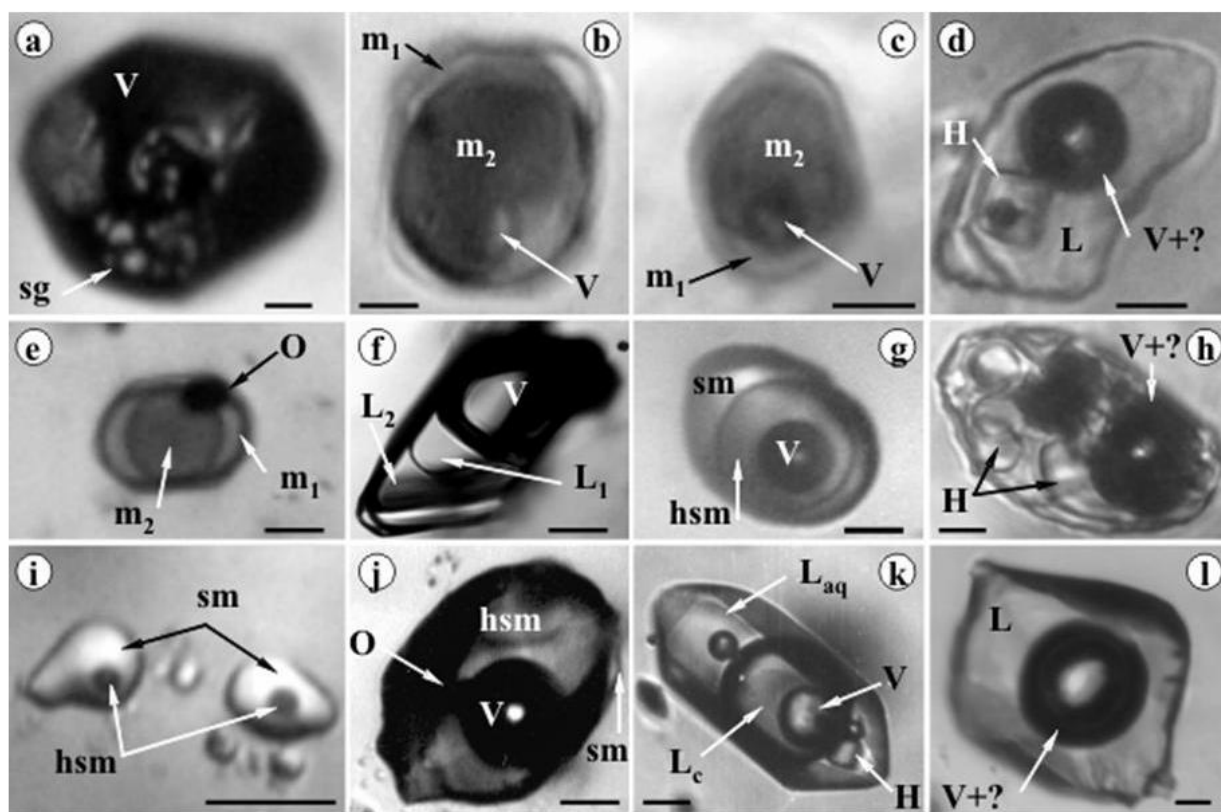
Figure 1. Selected types of fluid and melt inclusions from various geological formations from Romania, suggestive for immiscibility in various geological conditions; V- vapor, sg- “in situ” sublimated silicate roe, m 1 - acidic silicate melt, m 2 -mafic silicate melt, O- opaque, sm- silicate melt, hsm- hydrous saline melt, L 1 , - liquid hydrocarbon (?), L 2 , L aq - aqueous liquid, L c - CO 2 liquid, H- halite; a, b - Săpânta quartz xenoliths; c, k - Ditrău alkaline massif; e - Rosia Montana beta-quartz; g .- Deva “porphyry copper” deposit silicate melt - salt melt - vapor immiscibility at 1300^{\circ}\text{C} ; i . Th= 1085^{\circ}\text{C} in silicate melt and j . Th= 1086^{\circ}\text{C} in contemporaneous hydrous salt melt inclusion trapped in quartz; f . Bocșa-Săcărâmb epithermal ore deposit; d, h . a rind around the vapour bubble (pin point) together with solid microphase(s) at T = 25^{\circ}\text{C} ( d ) and around 400^{\circ}\text{C} ( h ), suggesting a second immiscible Fe-rich chloride (ferric) phase inside the brine inclusions in porphyry copper from Bolcana ( d ) and Rosia Poieni ( h ); Carbonic liquid- like phase (or a rind of reaction between aqueous vapour interface) around vapour bubble in aqueous inclusion from the miarolitic quartz from Vlădeasa granite. Scale bar: a, b, c, d, e, g, h, i, j, k, l - 10\mu\text{m} ; f- 70\mu\text{m} .
