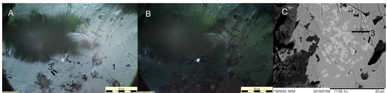
Fig. 5. Pearceite-polybasite (1) containing argentic fahlore (2) inclusions and overgrowths, as well as benleonardite blebs (3). A. Polarized reflected light, oil immersion; B. Crossed polarizers; C. Enlarged BSE image of a detail of the same field.
