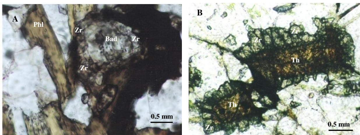
Fig. 3. Baddeleyite (Bad, big grain, centre, grayish white, clean, high refringence) with many small zircons around (Zr, grey), as a fringe, associated with phlogopite (Phl), and other new zircon grains around, NII sample G11-2-1/1 (A); Thorogummite (Th, yellow brown prismatic grain) with new small grains zircon (Zr) around, as a fringe, NII, sample G11-2/11 (B).
