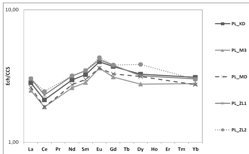
Figure 3: Spectra of REE distribution in washed ore normalized to upper continental crust.
