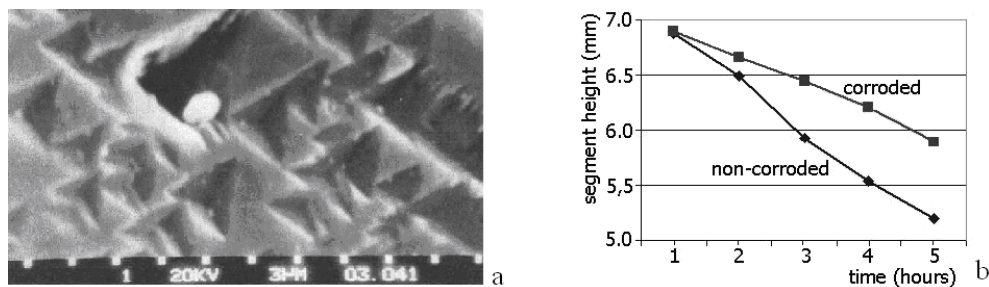
Fig.5. a. SEM micrograph of a corroded crystal face; b. improved wear resistance of cutting segments (Ruşchiţa marble)
