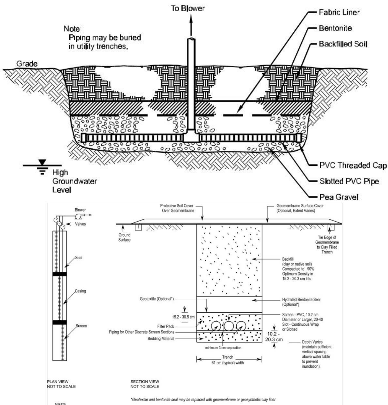
Typical construction scheme of a horizontal extraction well, view in plan and in section
